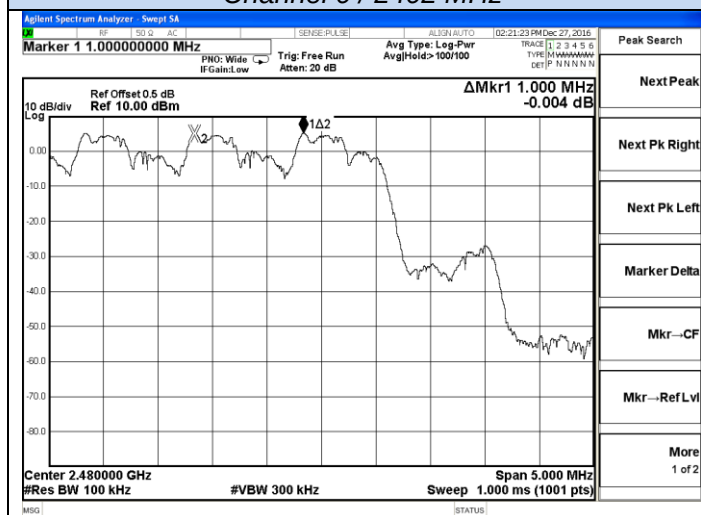
Channel 78 / 2480 MHz
