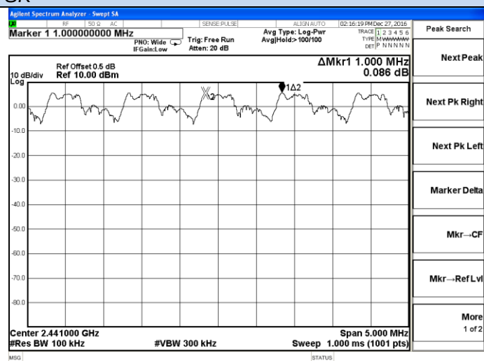
Channel 39 / 2441 MHz
