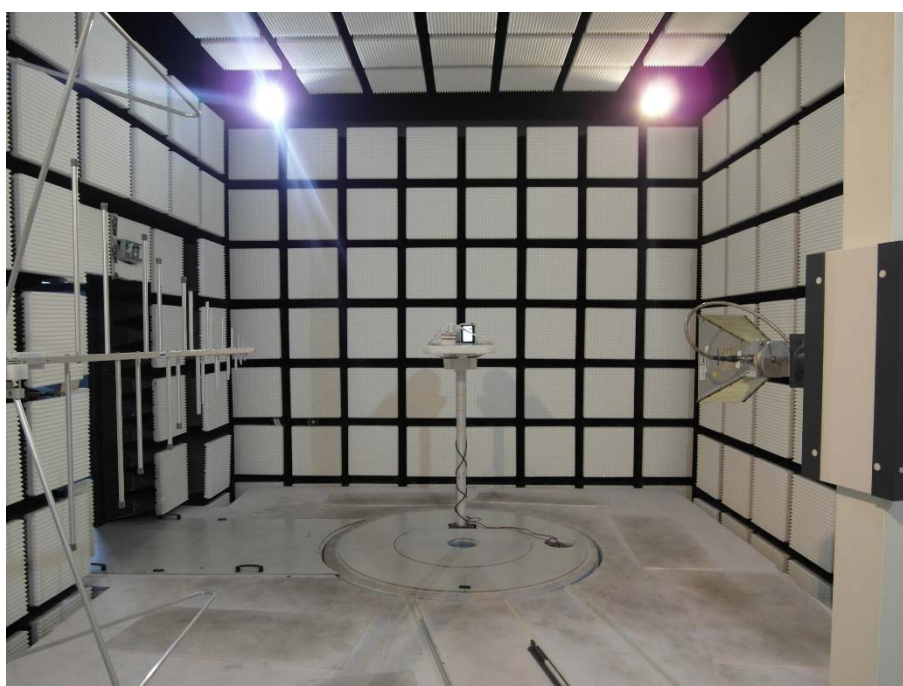
Photo 12: chamber C with antenna 2 setup
