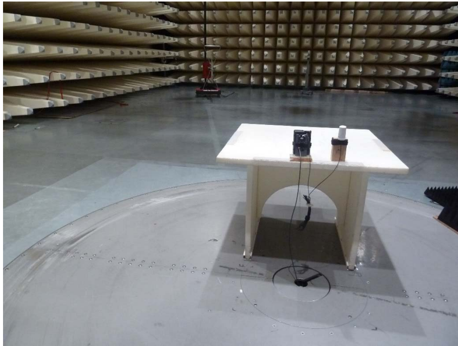
Photo 15: chamber F with antenna 2 setup
