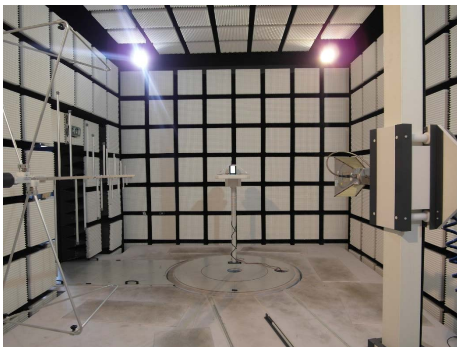
Photo 6: chamber C with antenna 1 setup
