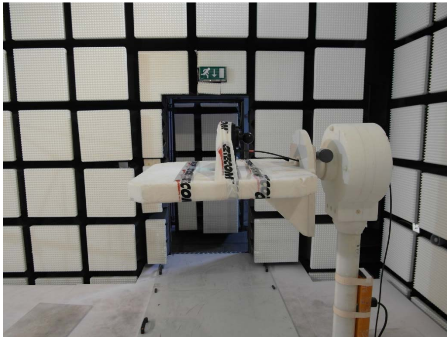
Photo 4: chamber C with antenna 1 setup
