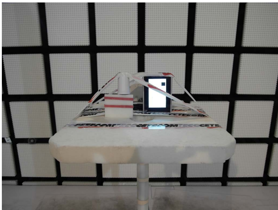
Photo 11: chamber C with antenna 2 setup
