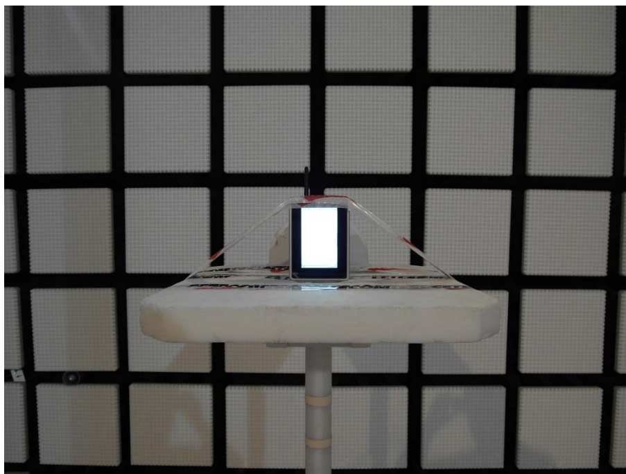
Photo 5: chamber C with antenna 1 setup
