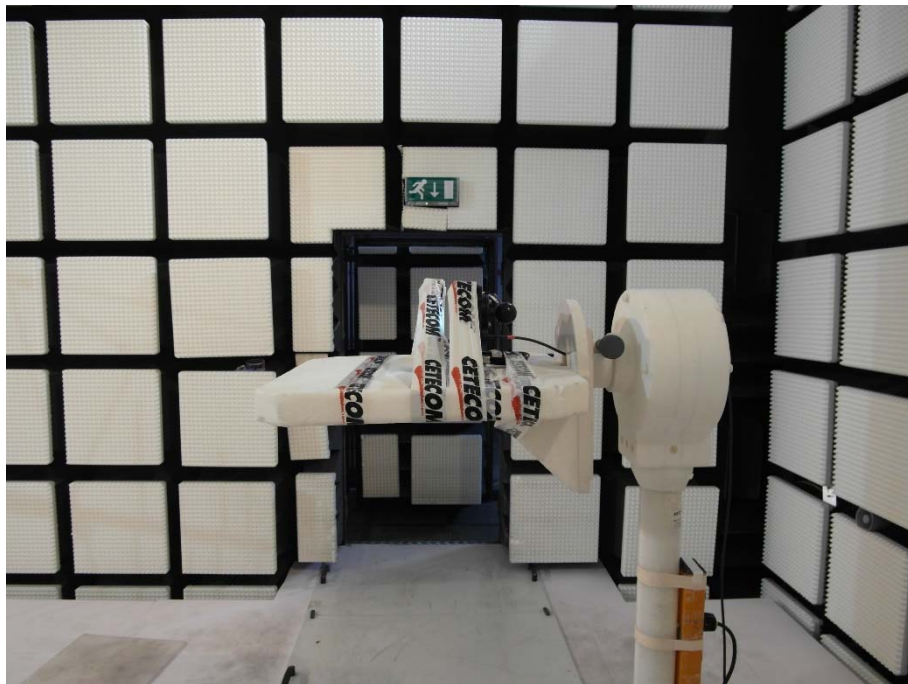
Photo 10: chamber C with antenna 2 setup
