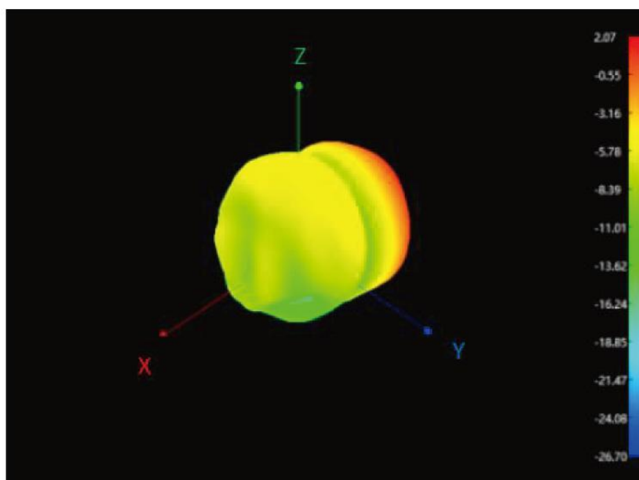
2440MHz 3D
