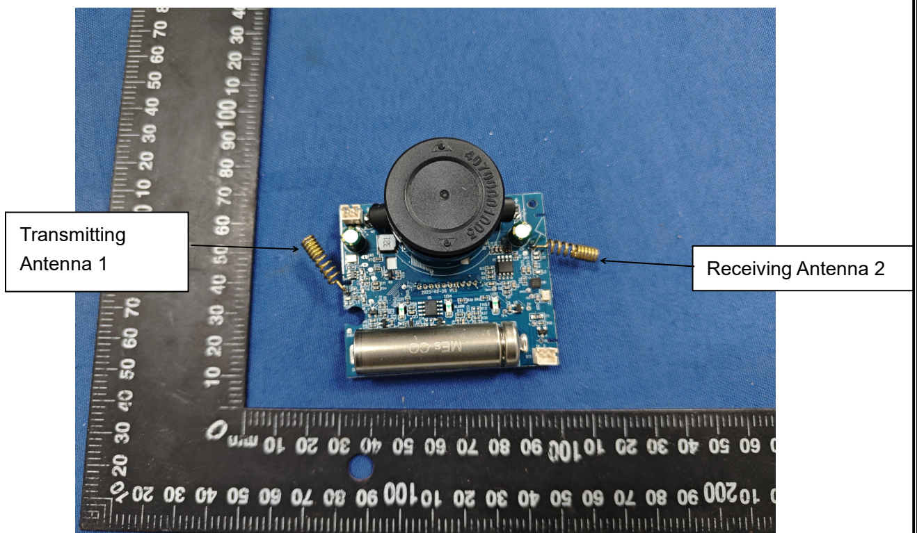
Fig.2 Antenna 2 is only receiving function(868.24MHz)
