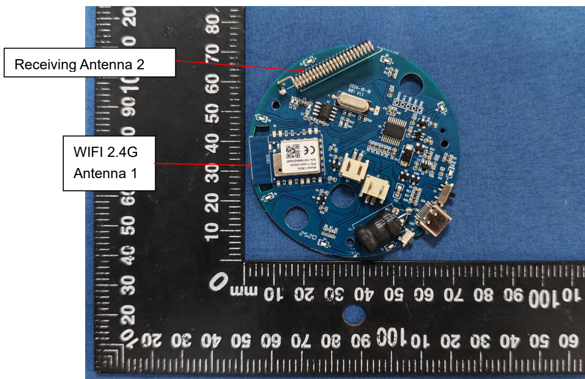
Fig.2 Antenna 2 is only receiving function(868.05MHz)
