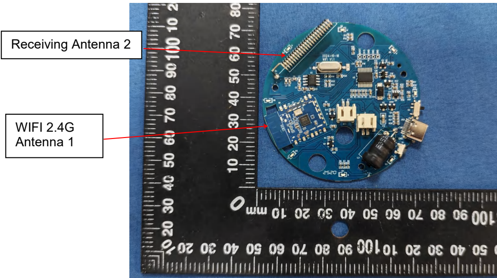
Antenna 2 is only receiving function(433.92MHz)
