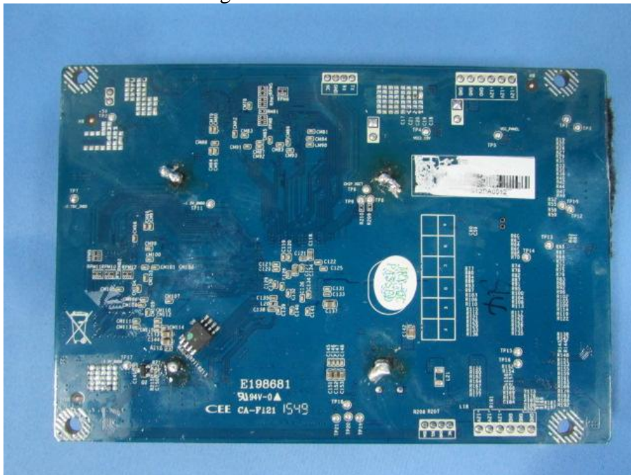
Signal Process Board view
