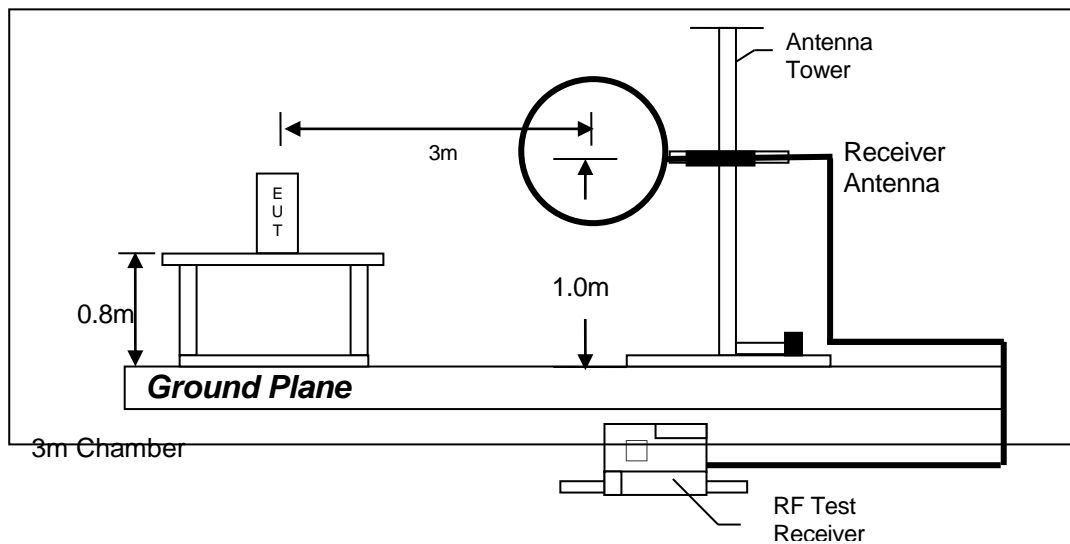
Test setup of radiated emissions up to 30MHz
