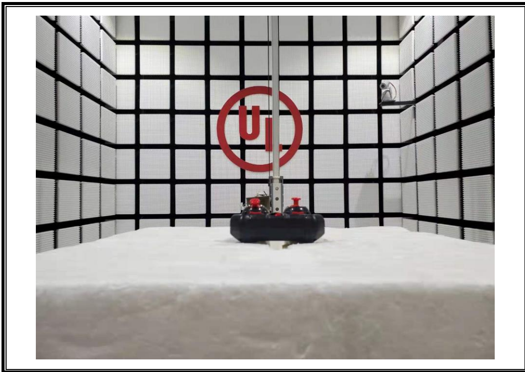
RADIATED RF MEASUREMENT SETUP (Above 1G – Y axis)
