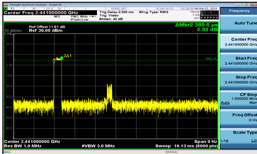
2DH1-Ant1-Hop-PASS
