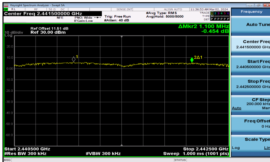
3DH5-Ant1-Hop-PASS
