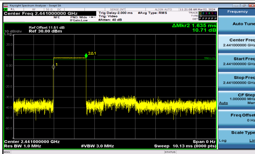
DH3-Ant1-Hop-PASS
