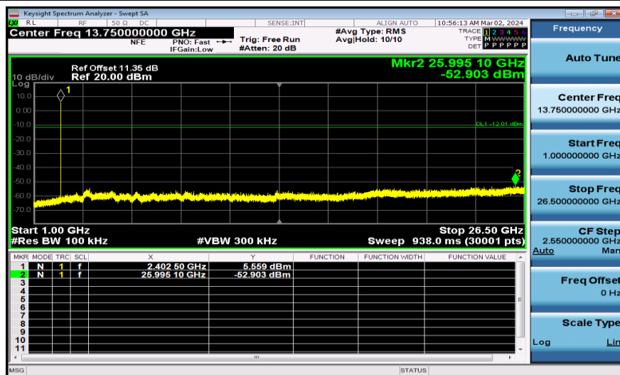
DH5-Ant1-2402-1000~26500-PASS
