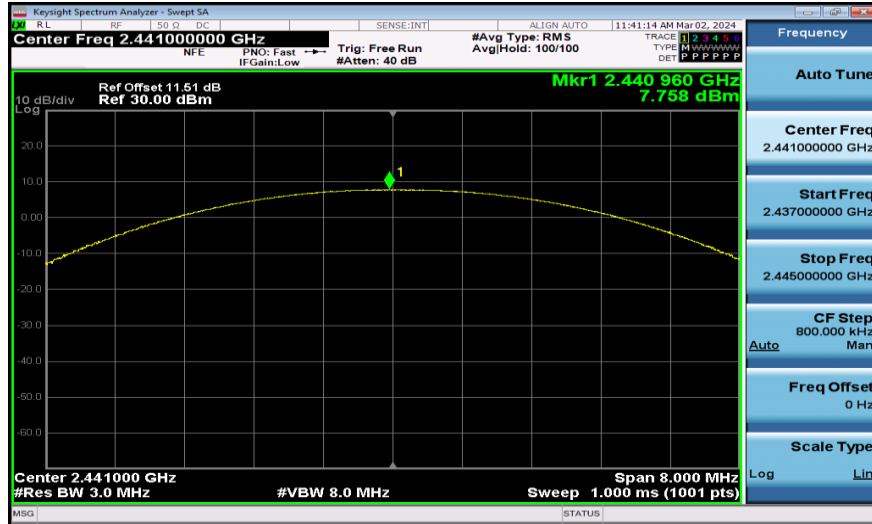
DH5-Ant1-2441-PASS
