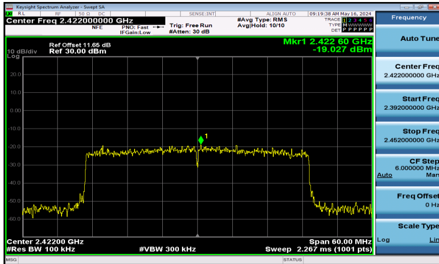
11AX40SISO-Ant1-2422-484Tone-0~Reference-PASS
