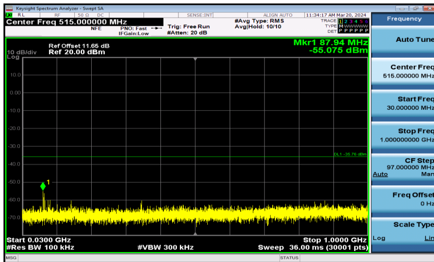
11AX20SISO-Ant1-2412-26Tone-30~1000-PASS
