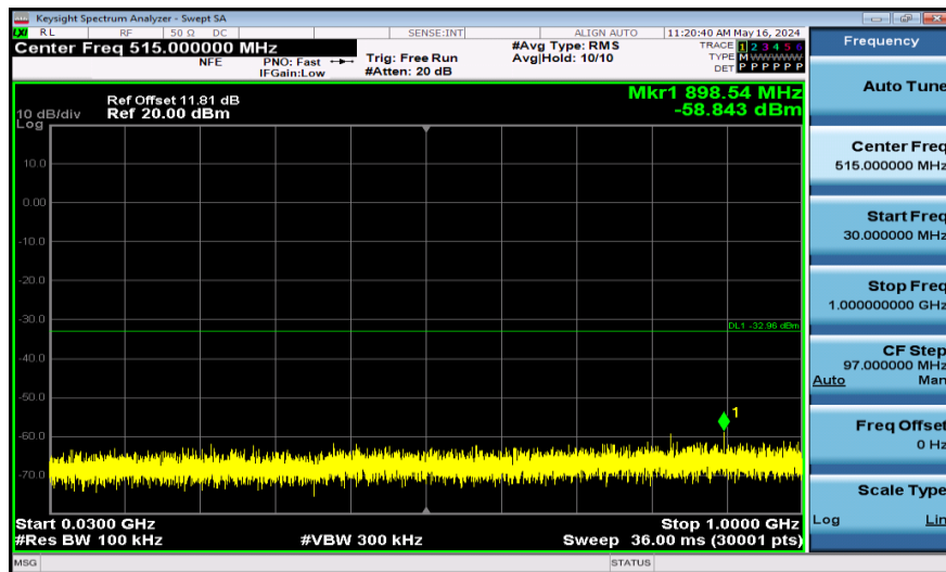
11AX20SISO-Ant1-2462-26Tone-30~1000-PASS
