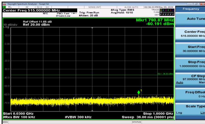
11AX40SISO-Ant1-2422-30~1000-PASS
