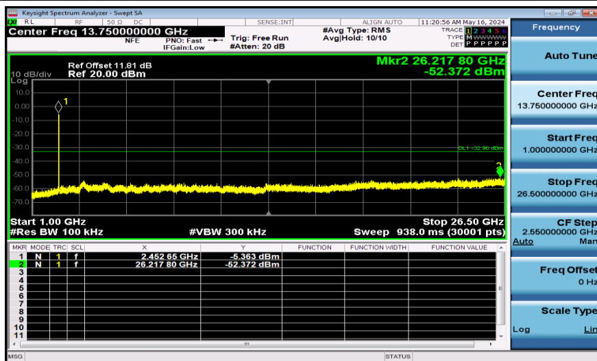
11AX20SISO-Ant1-2462-26Tone-1000~26500-PASS
