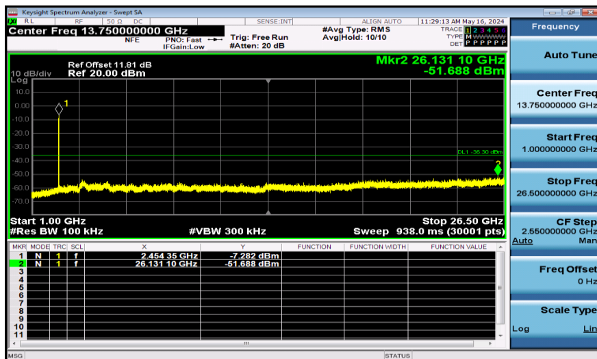
11AX20SISO-Ant1-2462-52Tone-1000~26500-PASS
