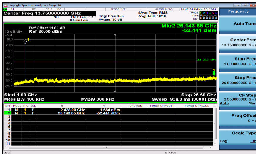
11AX20SISO-Ant1-2437-52Tone-1000~26500-PASS
