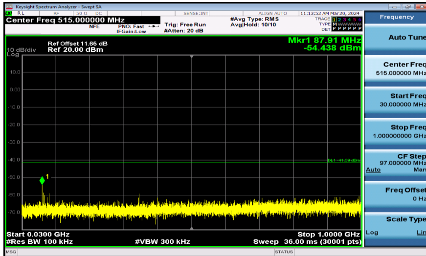
11AX20SISO-Ant1-2412-106Tone-30~1000-PASS
