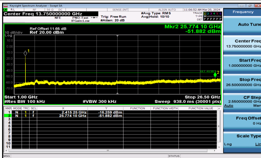
11AX20SISO-Ant1-2412-242Tone-1000~26500-PASS
