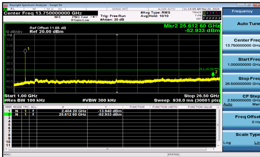
11AX20SISO-Ant1-2412-106Tone-1000~26500-PASS
