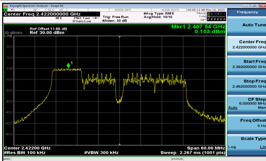
11AX40SISO-Ant1-2422-106Tone-0~Reference-PASS
