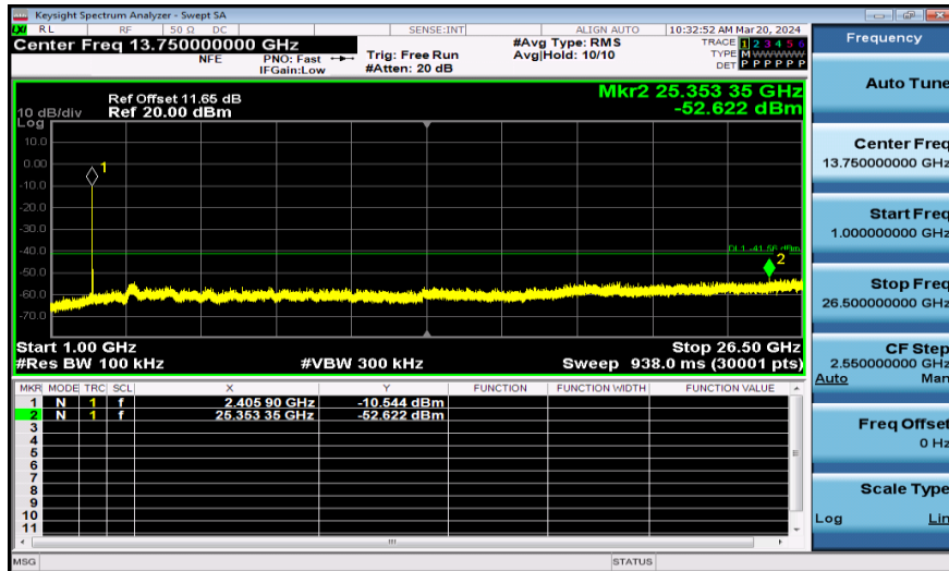
11AX20SISO-Ant1-2412-52Tone-1000~26500-PASS
