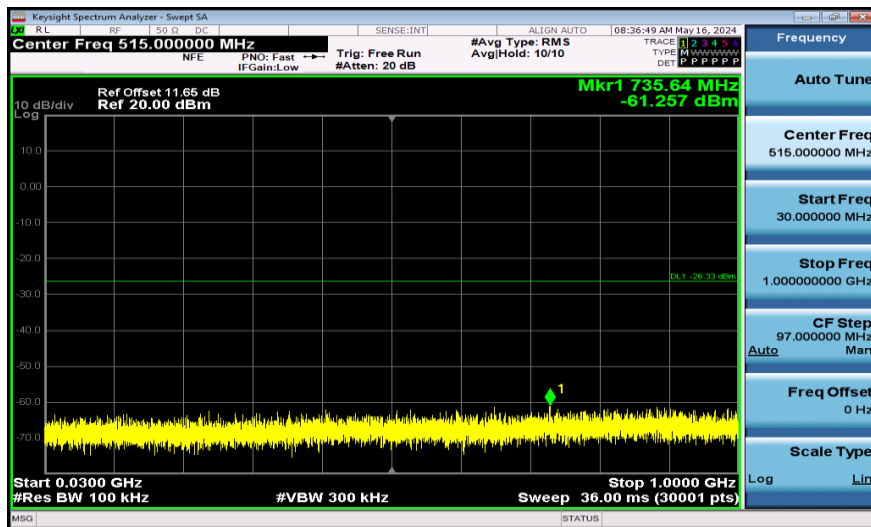
11AX40SISO-Ant1-2422-26Tone-30~1000-PASS
