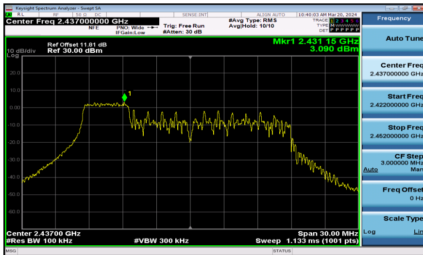
11AX20SISO-Ant1-2437-52Tone-0~Reference-PASS
