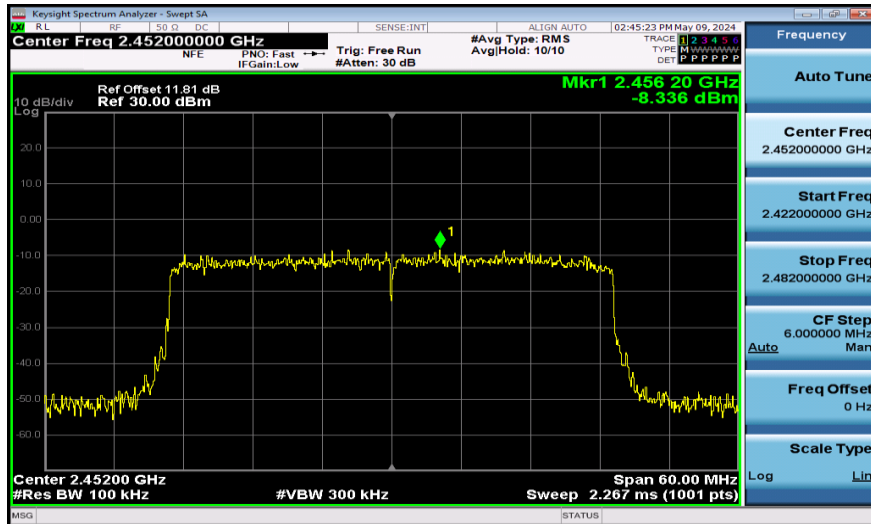
11AX40SISO-Ant1-2452-0~Reference-PASS
