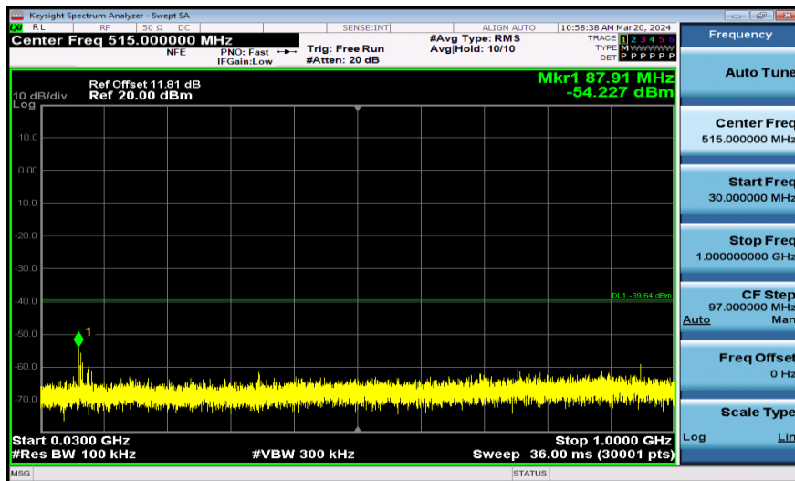
11AX20SISO-Ant1-2437-242Tone-30~1000-PASS
