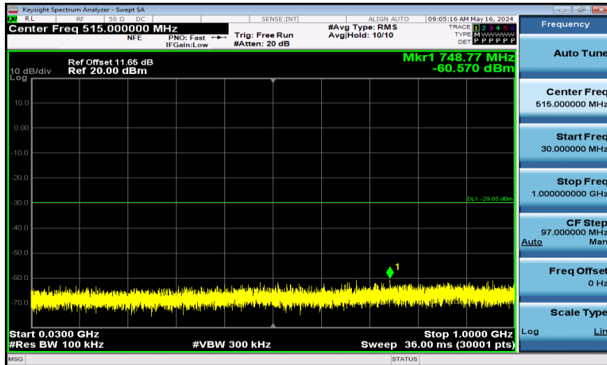
11AX40SISO-Ant1-2422-106Tone-30~1000-PASS
