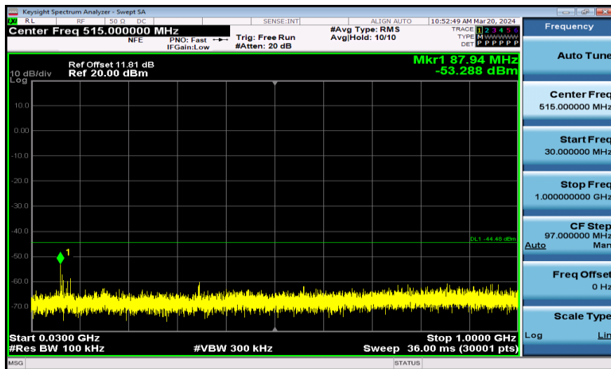
11AX20SISO-Ant1-2462-242Tone-30~1000-PASS
