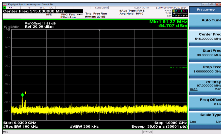
11AX20SISO-Ant1-2437-26Tone-30~1000-PASS
