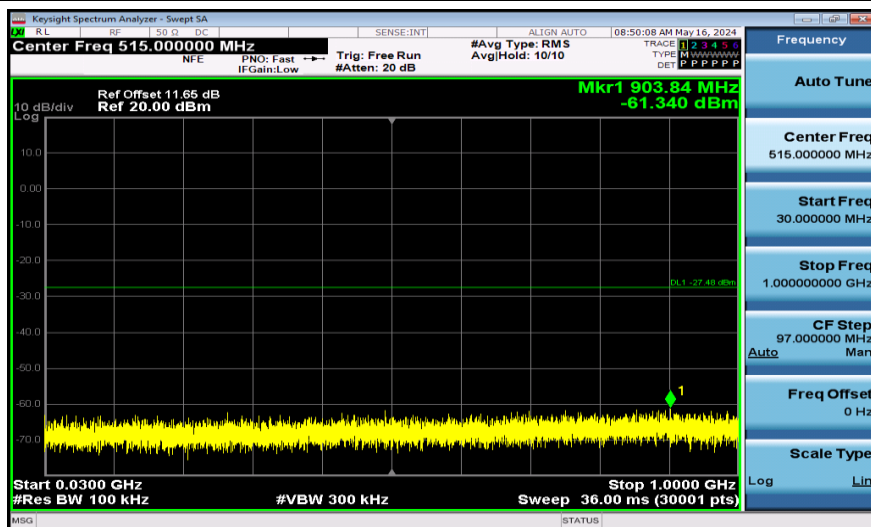
11AX40SISO-Ant1-2422-52Tone-30~1000-PASS
