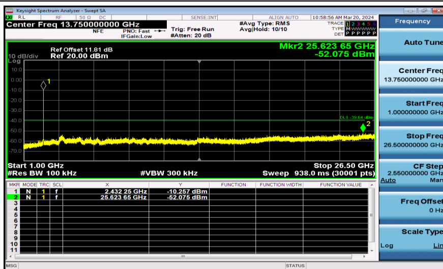
11AX20SISO-Ant1-2437-242Tone-1000~26500-PASS
