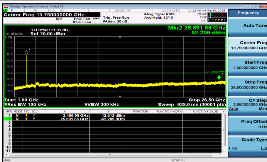
11AX20SISO-Ant1-2462-106Tone-1000~26500-PASS
