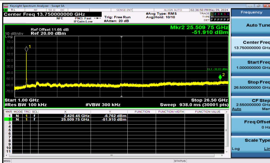
11AX40SISO-Ant1-2422-1000~26500-PASS
