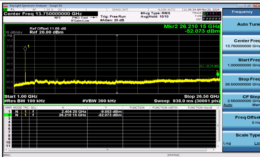
11AX20SISO-Ant1-2412-26Tone-1000~26500-PASS
