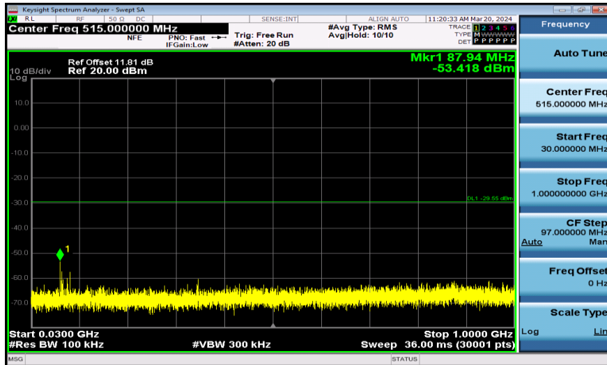
11AX20SISO-Ant1-2437-106Tone-30~1000-PASS
