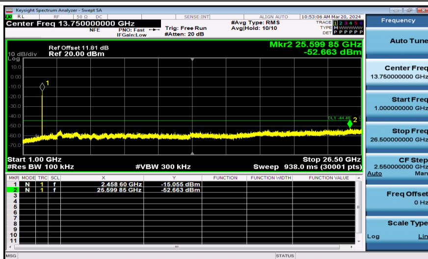
11AX20SISO-Ant1-2462-242Tone-1000~26500-PASS
