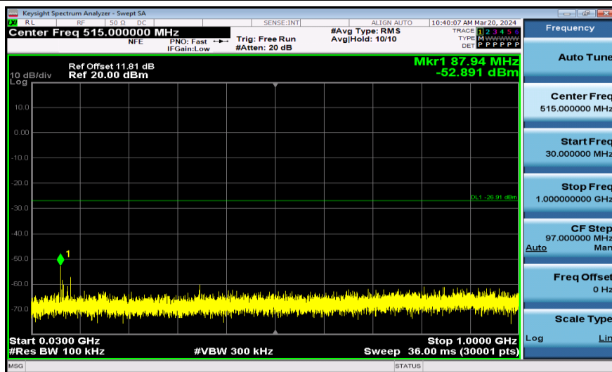
11AX20SISO-Ant1-2437-52Tone-30~1000-PASS
