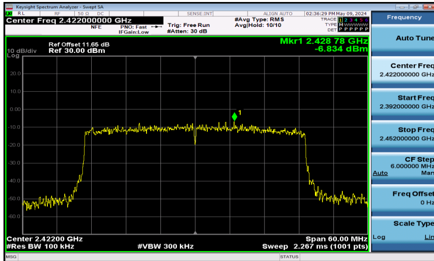
11AX40SISO-Ant1-2422-0~Reference-PASS
