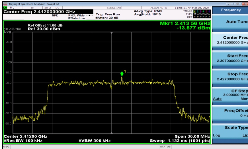
11AX20SISO-Ant1-2412-242Tone-0~Reference-PASS
