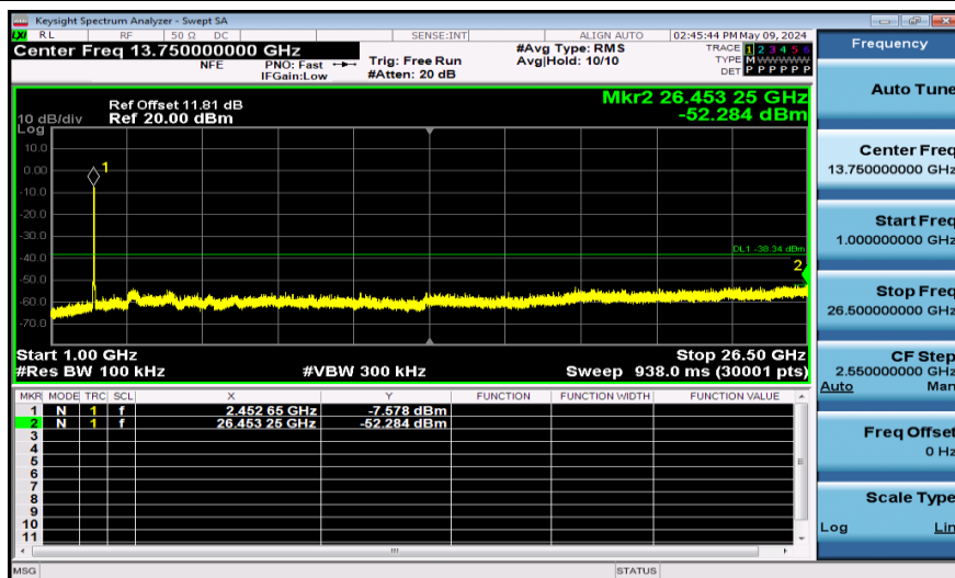
11AX40SISO-Ant1-2452-1000~26500-PASS
