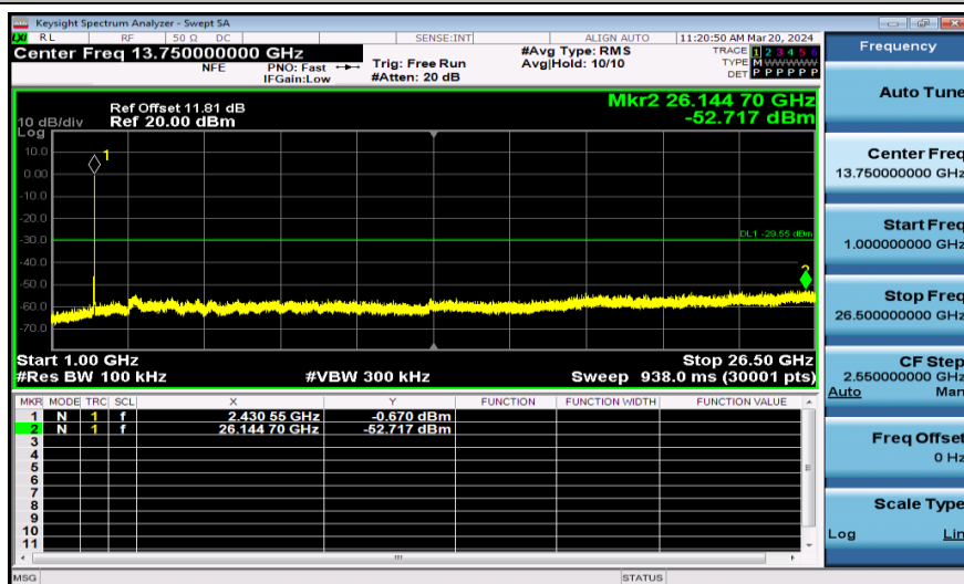
11AX20SISO-Ant1-2437-106Tone-1000~26500-PASS
