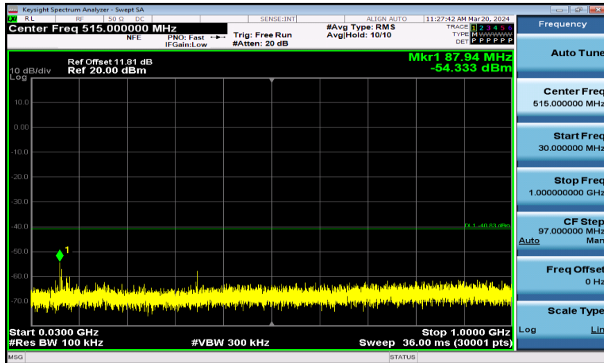
11AX20SISO-Ant1-2462-106Tone-30~1000-PASS
