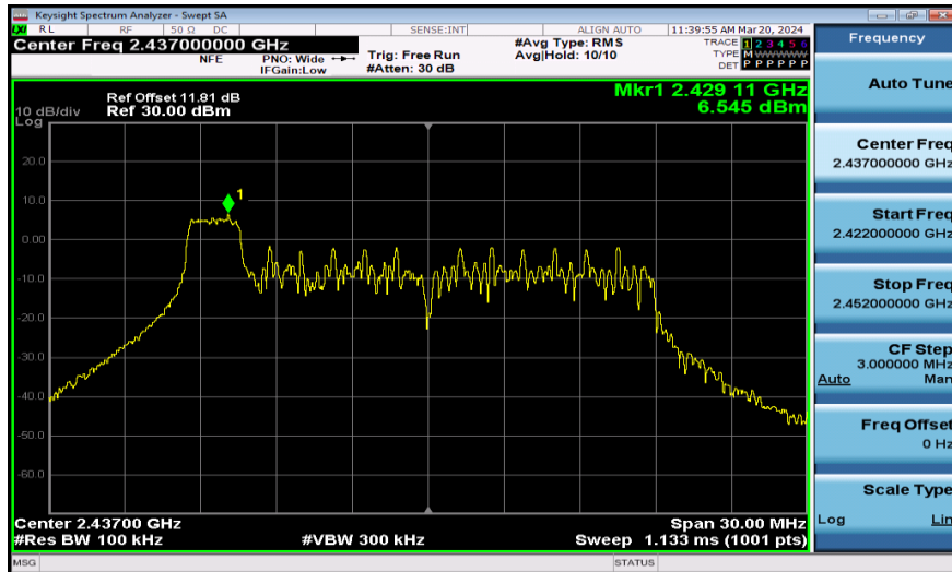
11AX20SISO-Ant1-2437-26Tone-0~Reference-PASS
