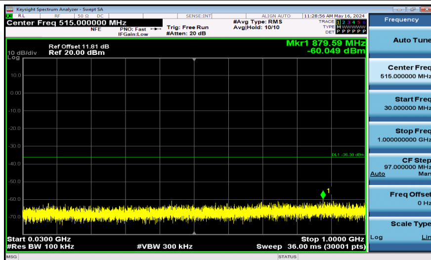
11AX20SISO-Ant1-2462-52Tone-30~1000-PASS
