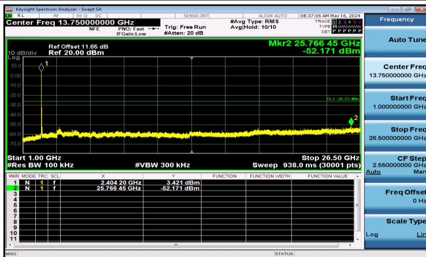
11AX40SISO-Ant1-2422-26Tone-1000~26500-PASS
