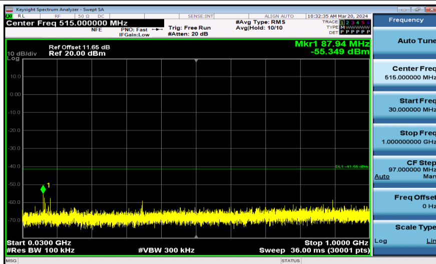
11AX20SISO-Ant1-2412-52Tone-30~1000-PASS
