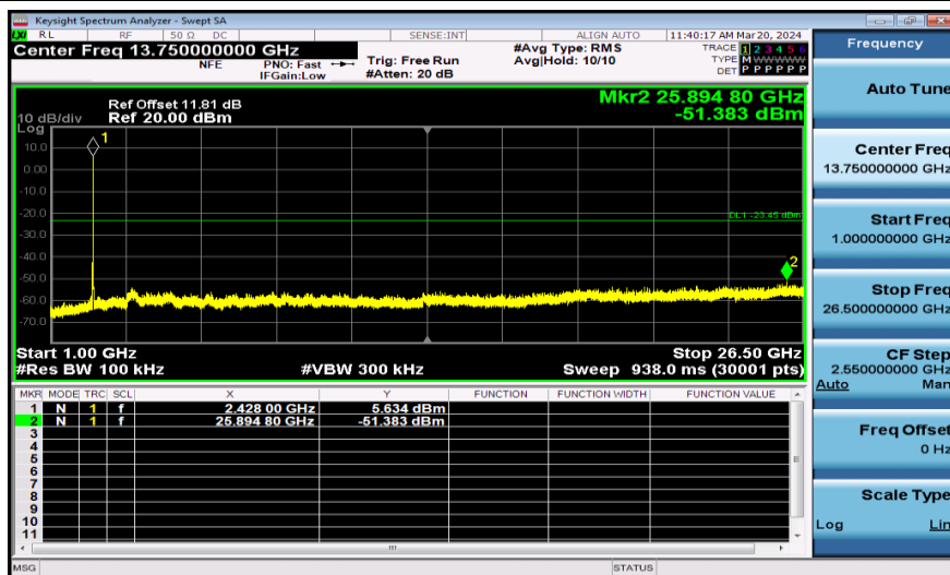
11AX20SISO-Ant1-2437-26Tone-1000~26500-PASS
