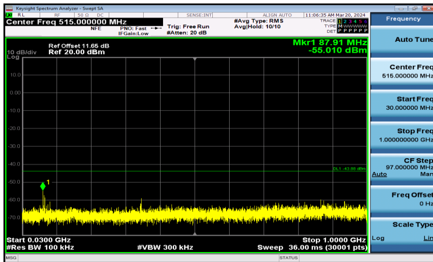
11AX20SISO-Ant1-2412-242Tone-30~1000-PASS
