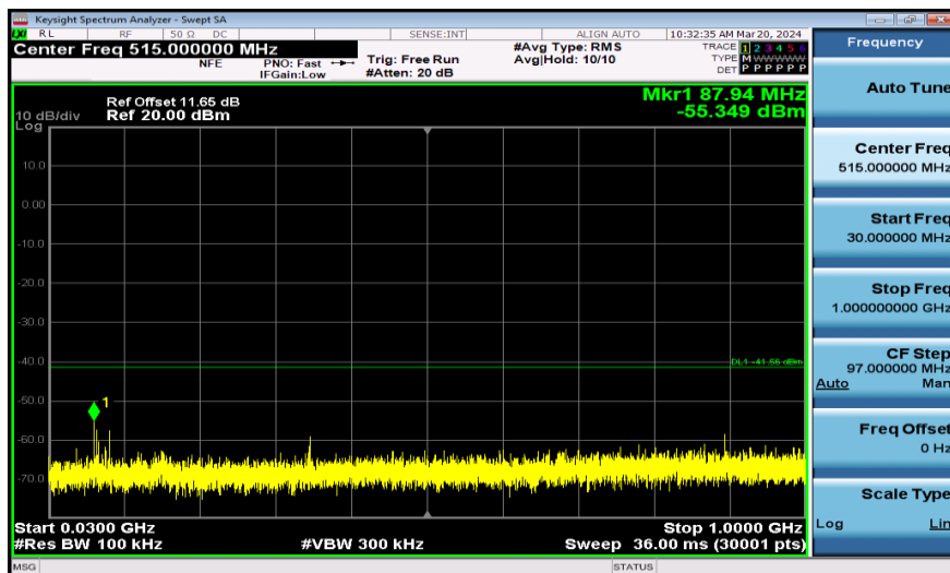
11AX20SISO-Ant1-2412-52Tone-30~1000-PASS
