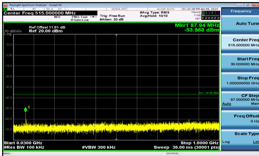
11AX40SISO-Ant1-2437-30~1000-PASS
