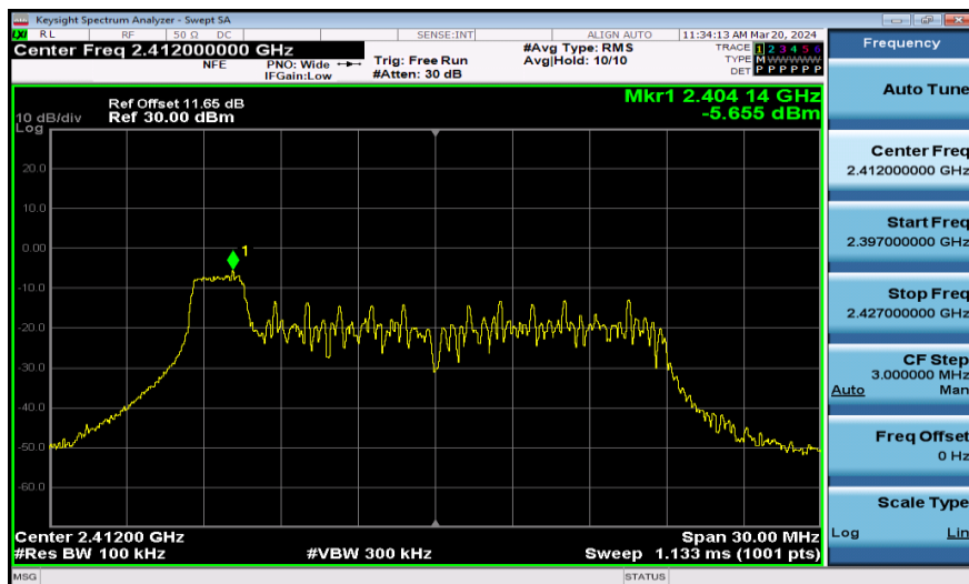
11AX20SISO-Ant1-2412-26Tone-0~Reference-PASS
