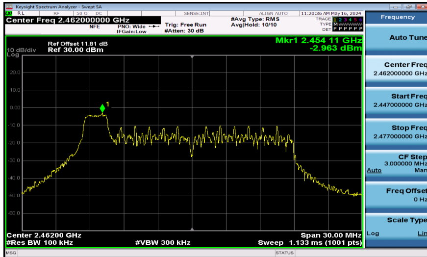
11AX20SISO-Ant1-2462-26Tone-0~Reference-PASS
