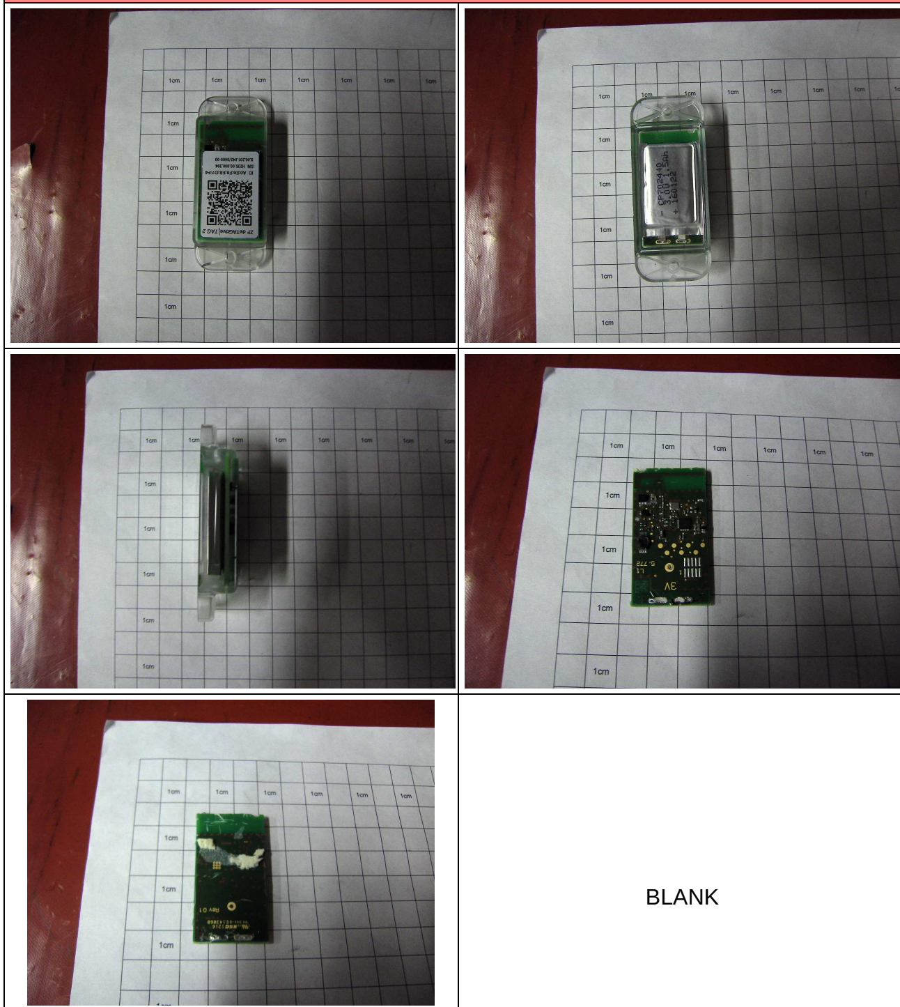
PHOTO N°1 – EUT IDENTIFICATION
