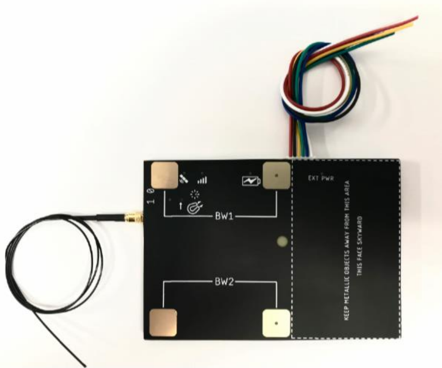
EUT Front View with VHF Antenna and Break Out Pigtail
