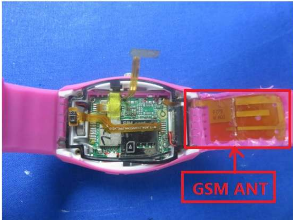
Fig.14.1 EUT Antenna Locations
