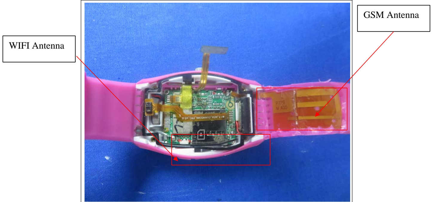
Antenna View
