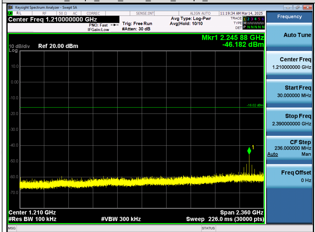
Test Graph EDR ANT1 2402 3Mbps Lower Band Emissions
