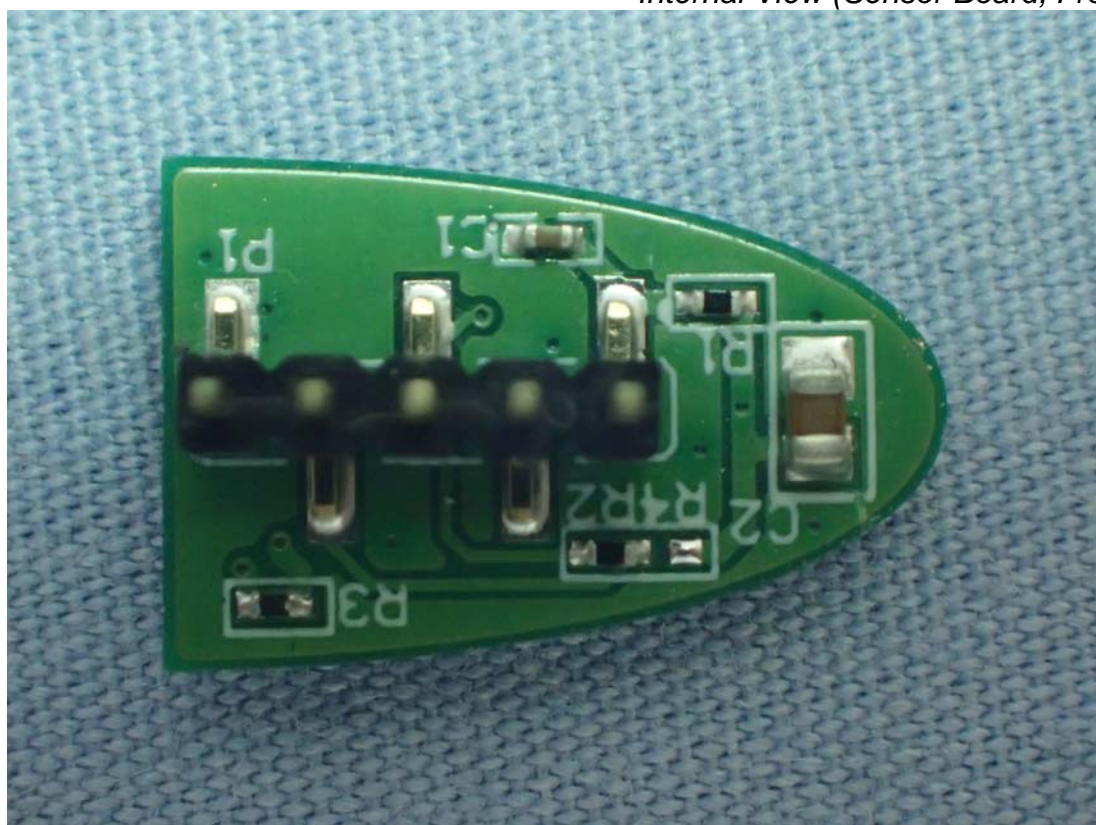
Figure 12 Internal View (Sensor Board, Front View)
