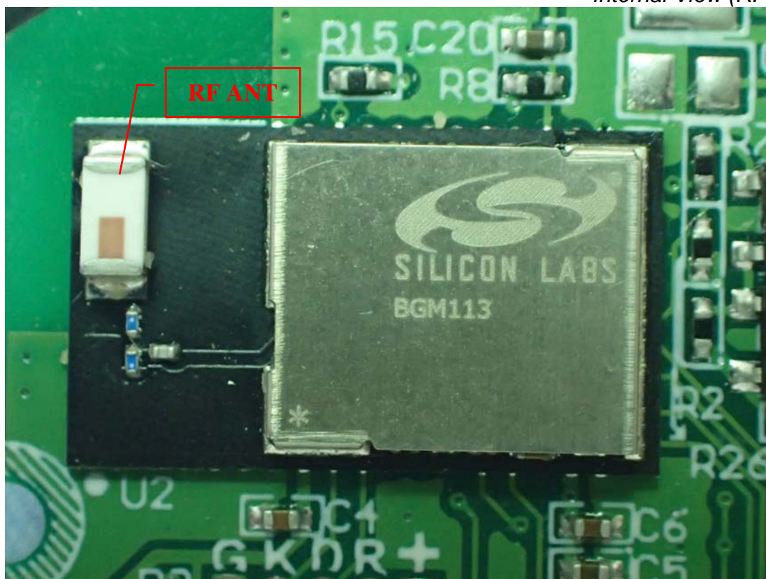
Figure 11 Internal View (RF Module)
