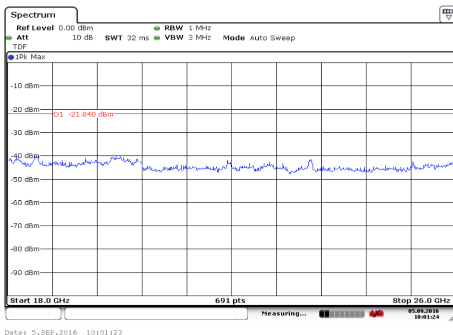
Fig. 49 Conducted Spurious Emission (All channel, 18 GHz-26 GHz)
