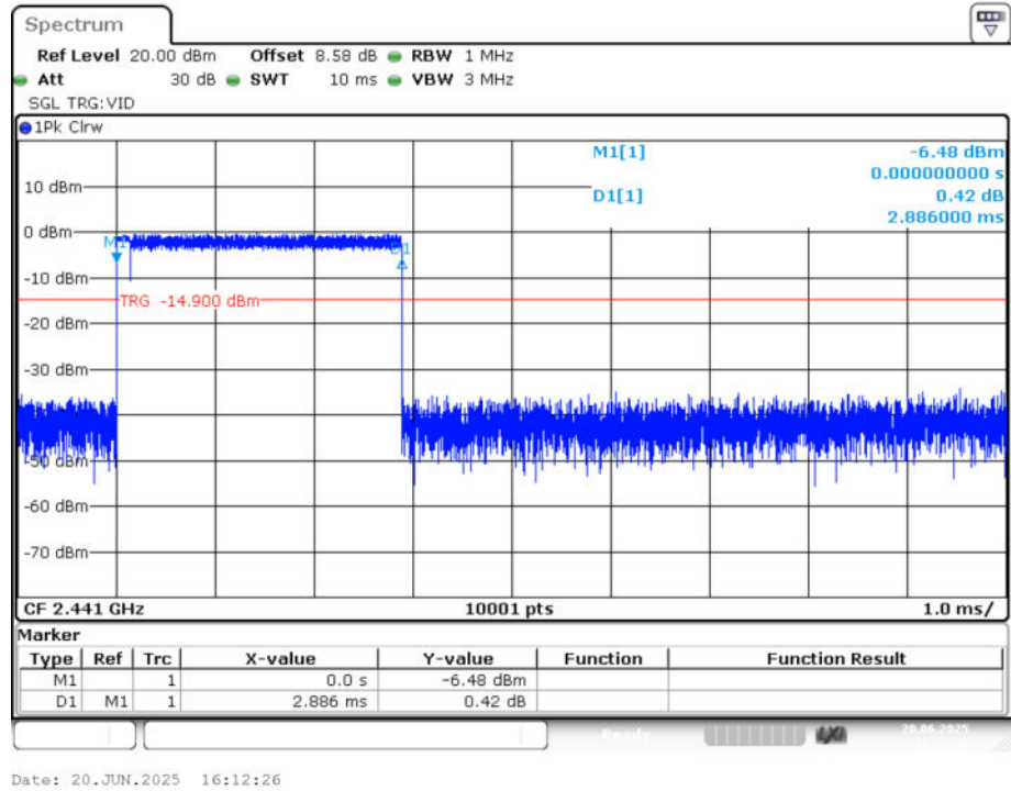
Dwell NVNT 2-DH5 2441MHz Ant1 Accumulated
