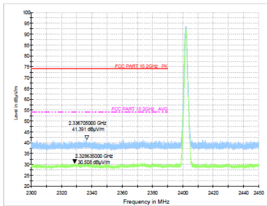
Test Mode: \pi/4 DQPSK-Low Hopping-off
