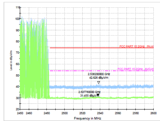
Test Mode: \pi/4 DQPSK-High Hopping-on
