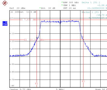
26 dB Bandwidth
