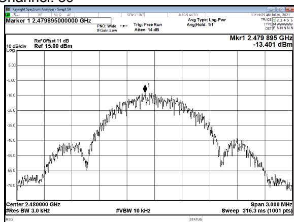
Modulation Standard: GFSK (1Mbps) Channel: 39
