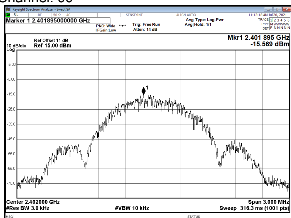
Modulation Standard: GFSK (1Mbps) Channel: 00
