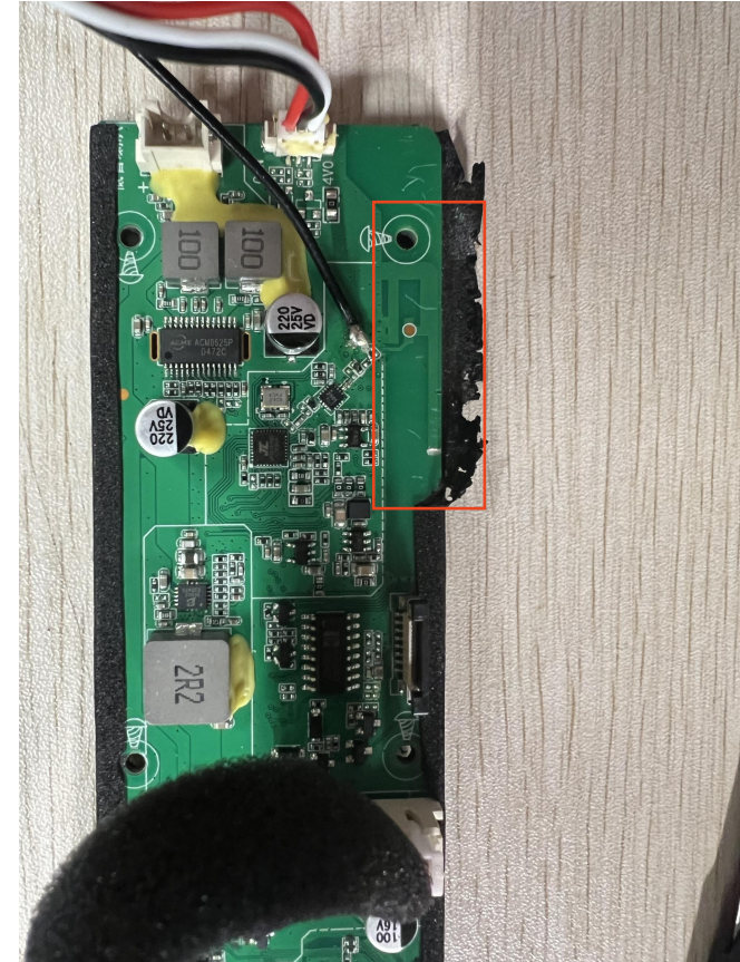
Antenna close-up
