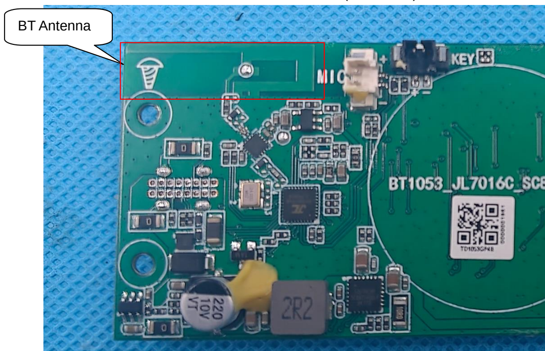
INTERNAL VIEW OF EUT (FIGURE 8)
