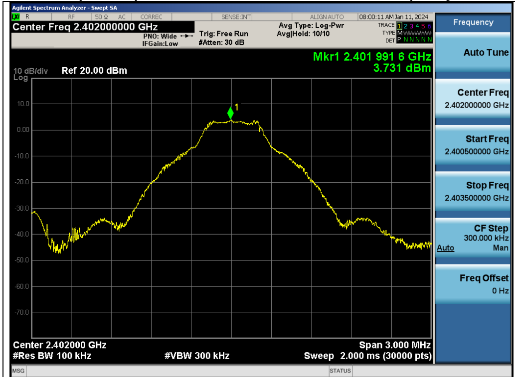
Test_Graph_BR_ANT1_2402_1Mbps_Reference Level
