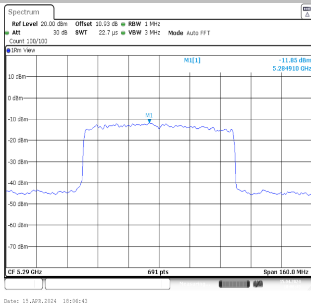
11AX80MIMO-Ant2-5290-PASS
