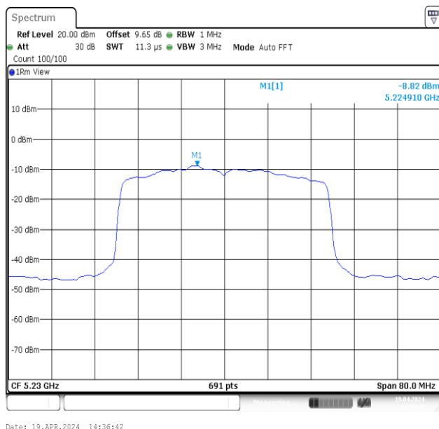
11AX40MIMO-Ant2-5230-PASS
