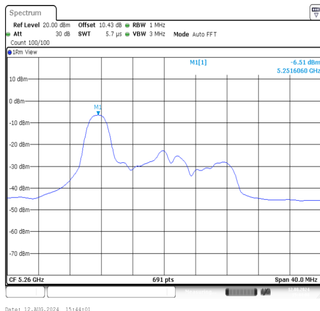
11AX20MIMO-Ant2-5260-26Tone-RU0-PASS
