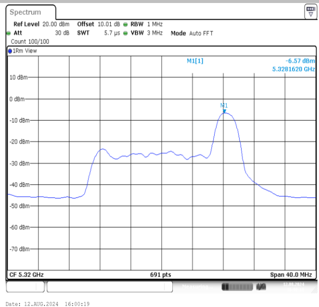
11AX20MIMO-Ant2-5320-26Tone-RU8-PASS
