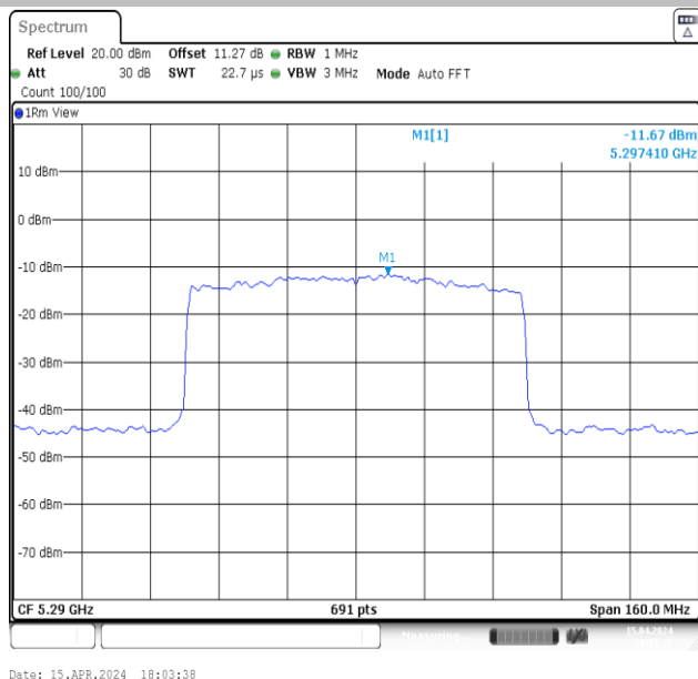
11AX80MIMO-Ant1-5290-PASS
