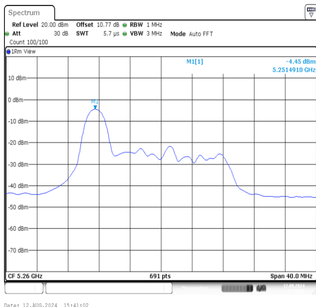
11AX20MIMO-Ant1-5260-26Tone-RU0-PASS
