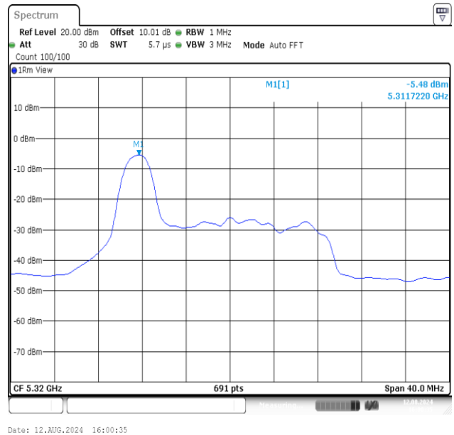
11AX20MIMO-Ant2-5320-26Tone-RU0-PASS
