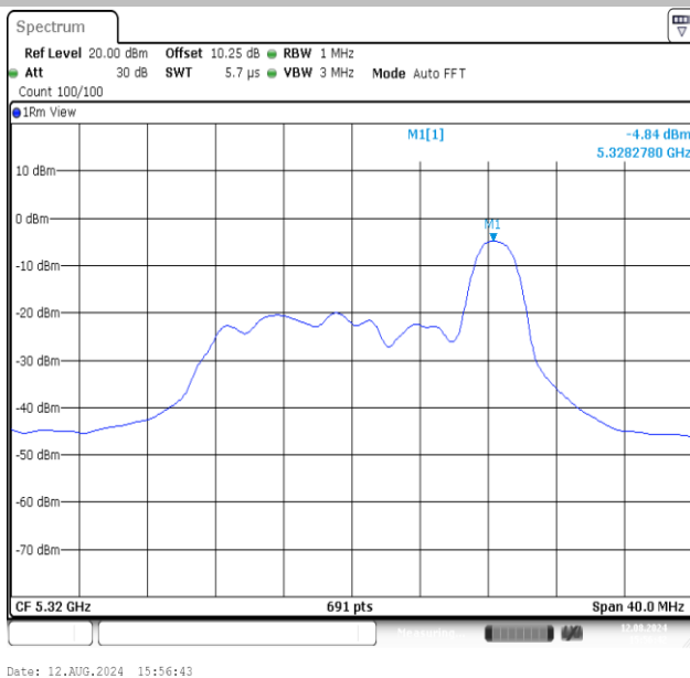
11AX20MIMO-Ant1-5320-26Tone-RU8-PASS
