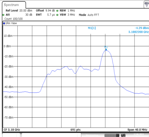
11AX20MIMO-Ant1-5180-26Tone-RU0-PASS
