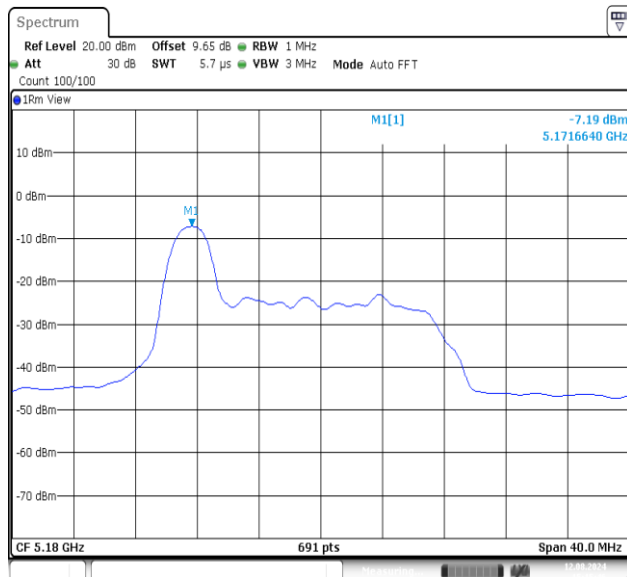
11AX20MIMO-Ant2-5180-26Tone-RU0-PASS
