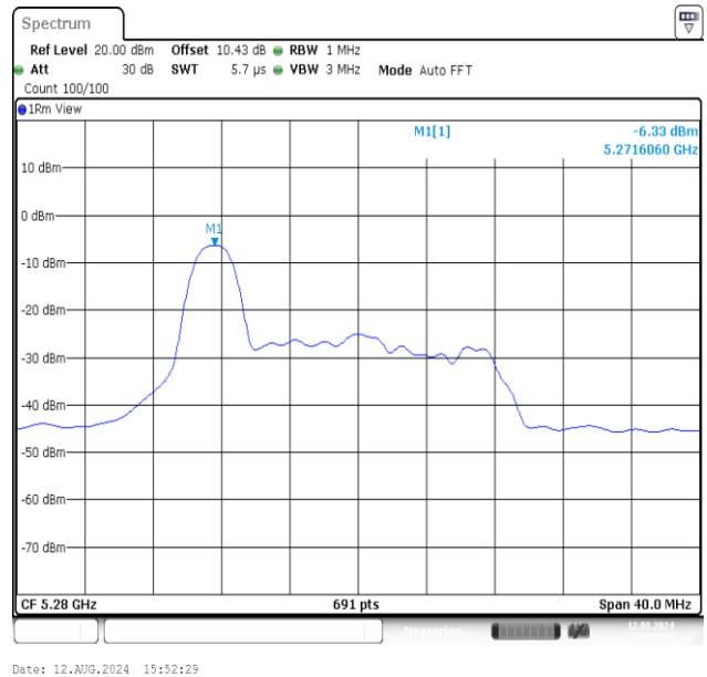
11AX20MIMO-Ant2-5280-26Tone-RU0-PASS
