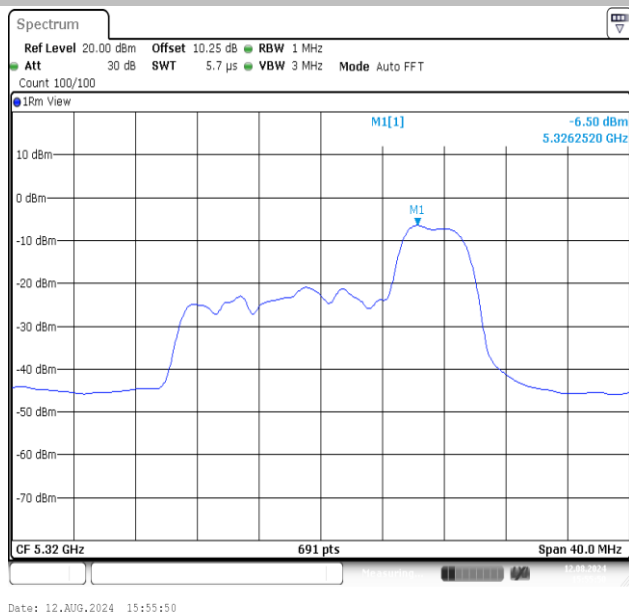
11AX20MIMO-Ant1-5320-52Tone-RU40-PASS
