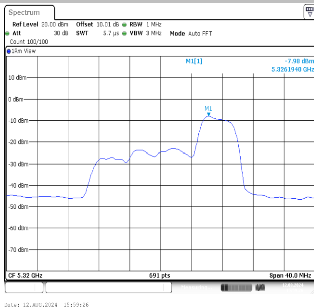
11AX20MIMO-Ant2-5320-52Tone-RU40-PASS
