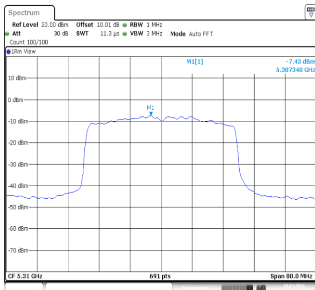
11AX40MIMO-Ant2-5310-PASS
