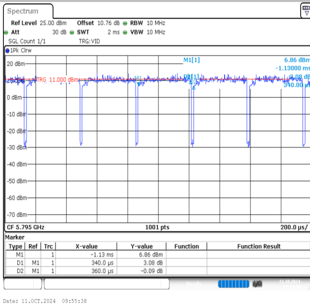
NTVN-11AC40MIMO-Ant1-5795
