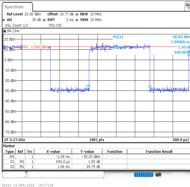
NTVN-11AX40MIMO-Ant1-5270
