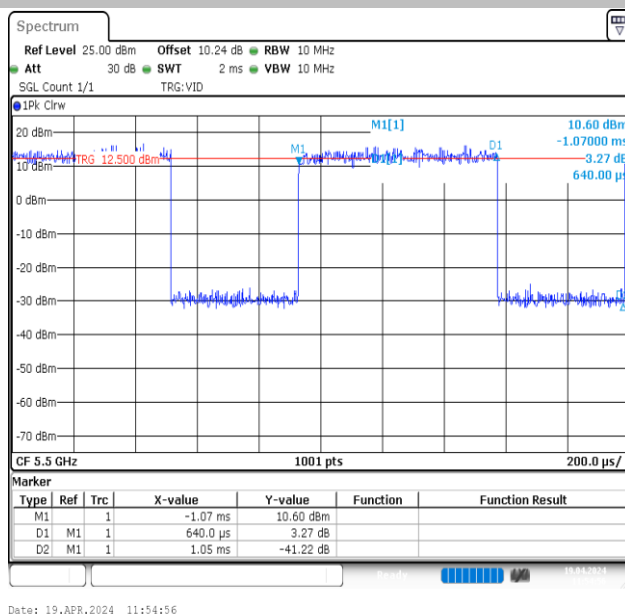
NTVN-11AX20MIMO-Ant2-5500
