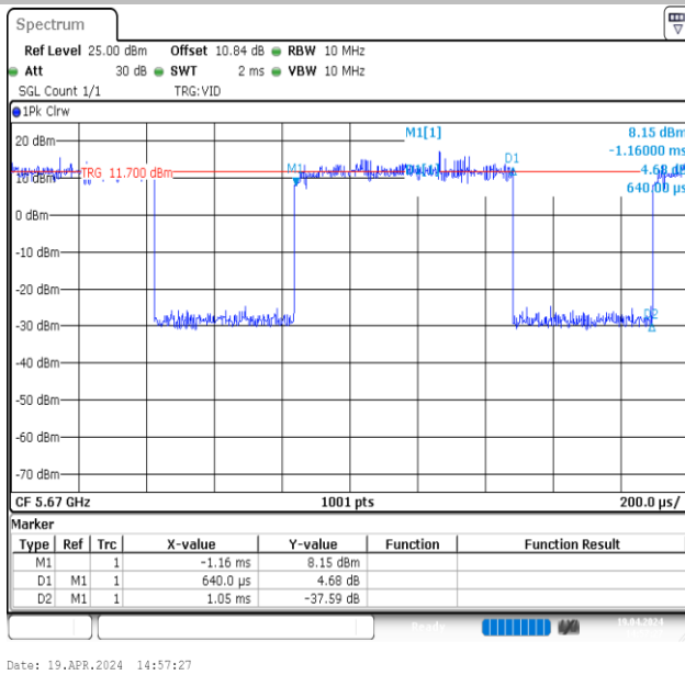
NTVN-11AX40MIMO-Ant1-5670
