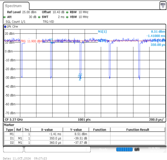
NTVN-11AC40MIMO-Ant2-5270
