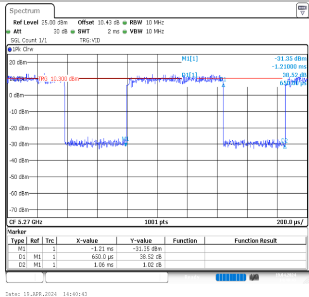
NTVN-11AX40MIMO-Ant2-5270
