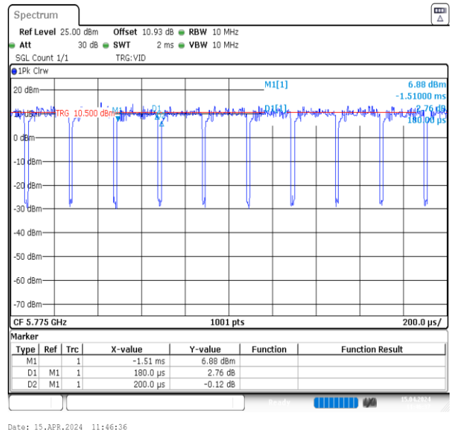
NTVN-11AC80MIMO-Ant2-5775
