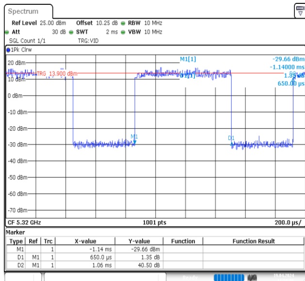
NTVN-11AX20MIMO-Ant1-5320
