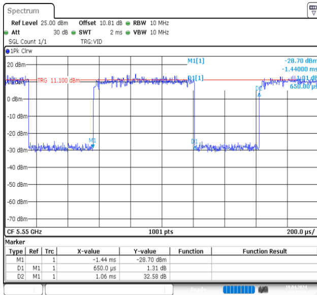
NTVN-11AX40MIMO-Ant1-5550
