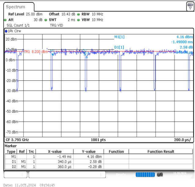
NTVN-11AC40MIMO-Ant2-5795
