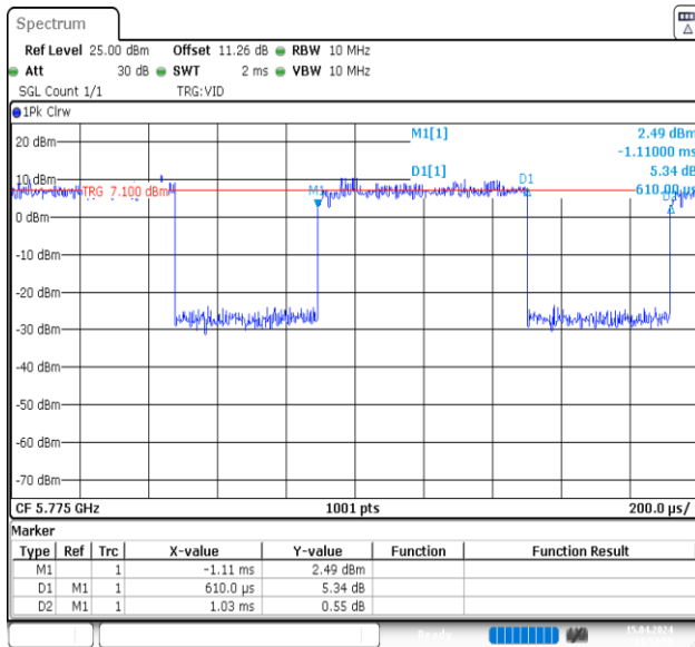
NTNV-11AX80MIMO-Ant1-5775
