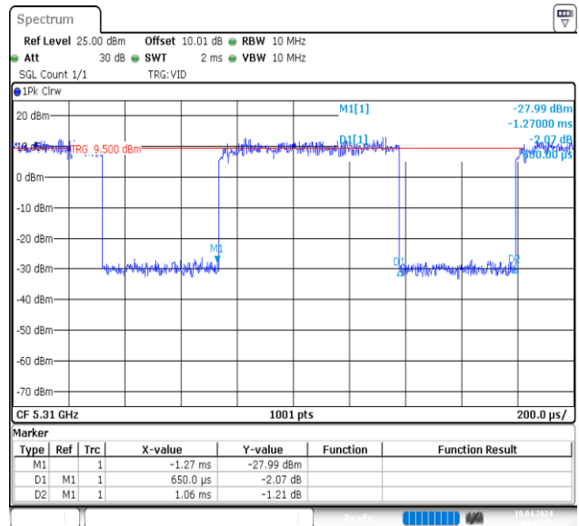
NTVN-11AX40MIMO-Ant2-5310
