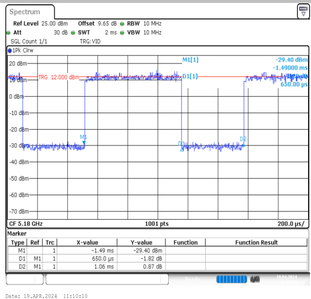
NTVN-11AX20MIMO-Ant2-5180
