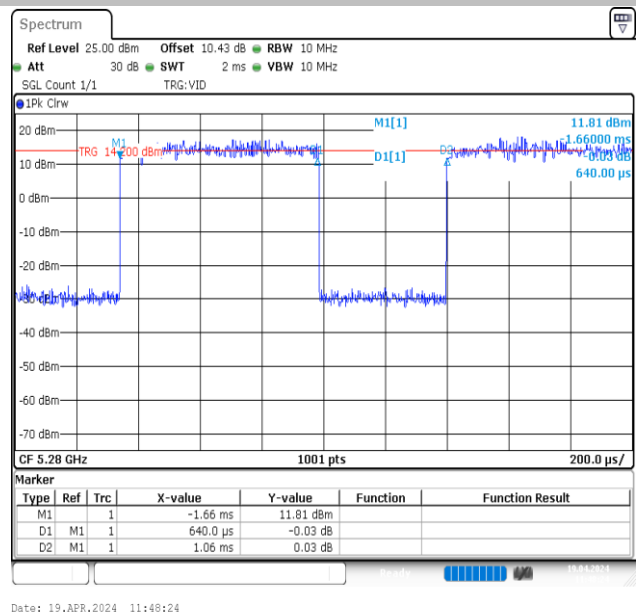
NTVN-11AX20MIMO-Ant2-5280
