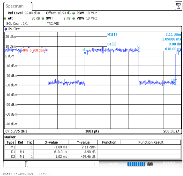
NTNV-11AX80MIMO-Ant2-5775
