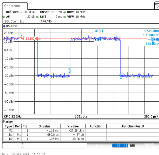
NTVN-11AX20MIMO-Ant2-5320
