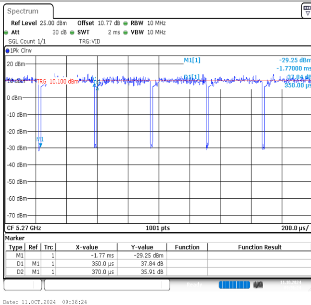
NTVN-11AC40MIMO-Ant1-5270
