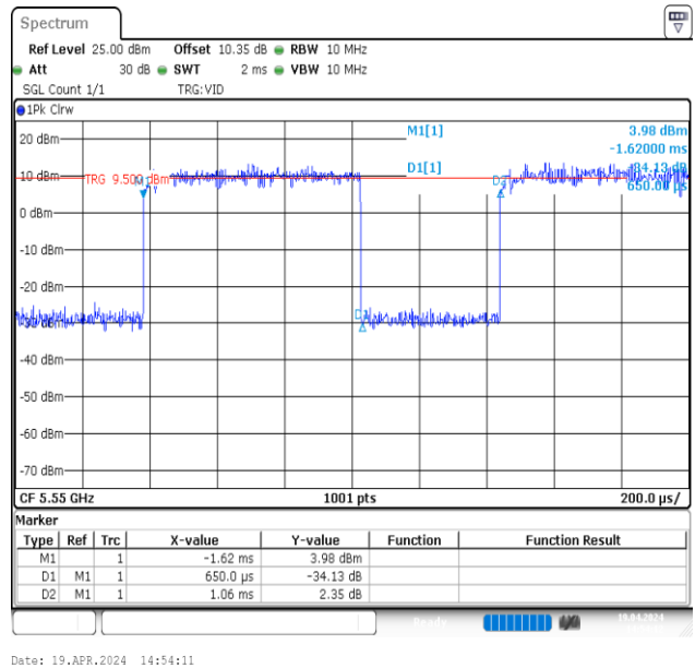
NTVN-11AX40MIMO-Ant2-5550
