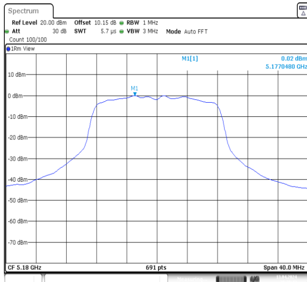
11A-Ant2-5180-PASS
