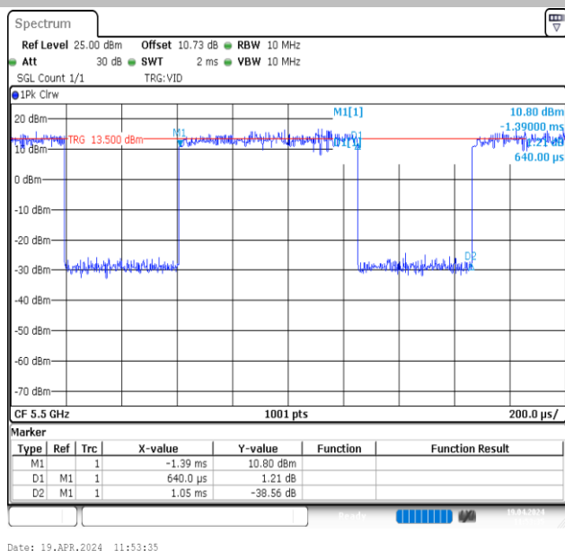
NTVN-11AX20MIMO-Ant1-5500
