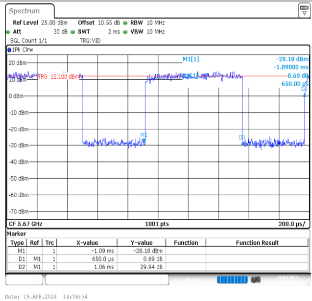
NTVN-11AX40MIMO-Ant2-5670
