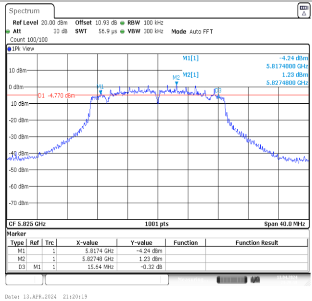
11N20MIMO-Ant2-5825-PASS
