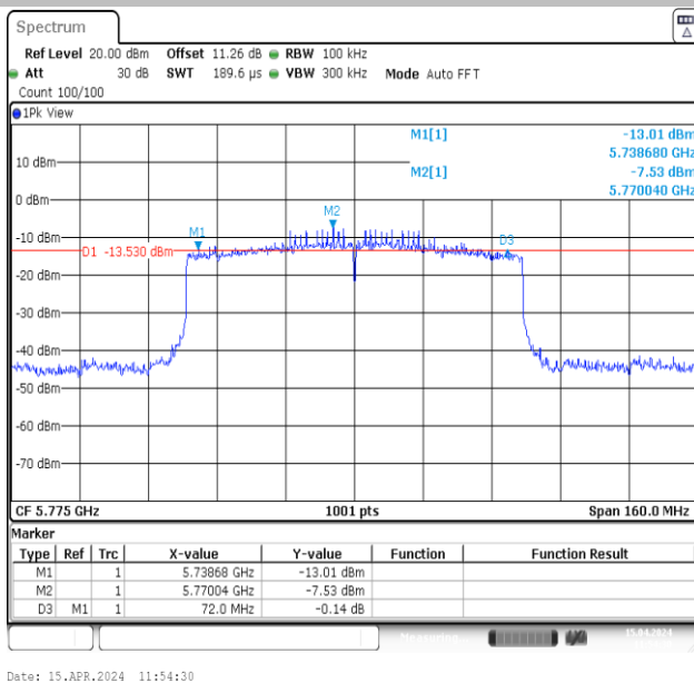
11AX80MIMO-Ant1-5775-PASS
