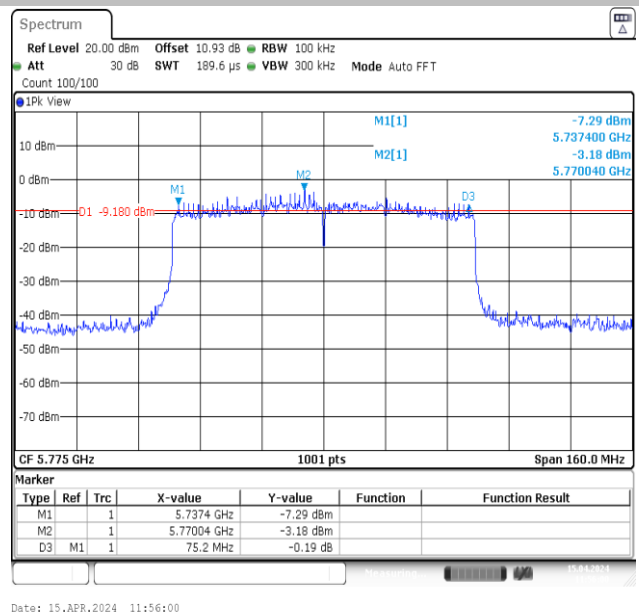
11AX80MIMO-Ant2-5775-PASS
