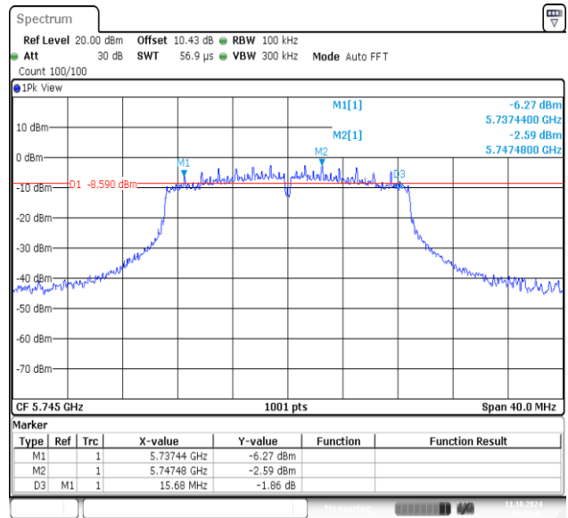
11AC20MIMO-Ant2-5745-PASS
