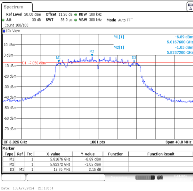
11N20MIMO-Ant1-5825-PASS
