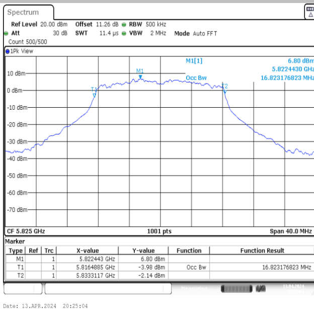
11A-Ant1-5825
