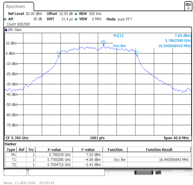
11A-Ant2-5785
