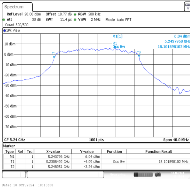
11AC20MIMO-Ant1-5240
