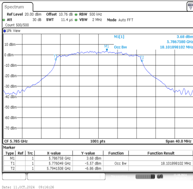
11AC20MIMO-Ant1-5785
