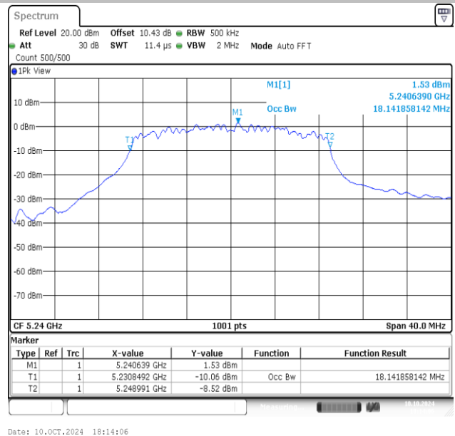
11AC20MIMO-Ant2-5240
