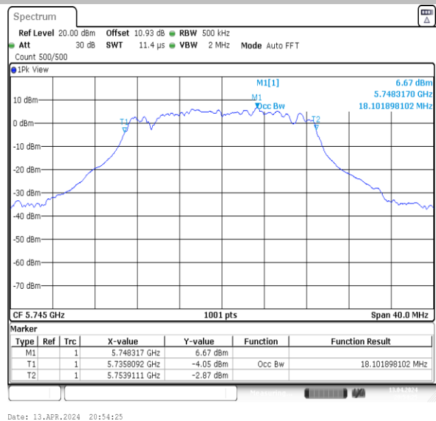
11N20MIMO-Ant2-5745
