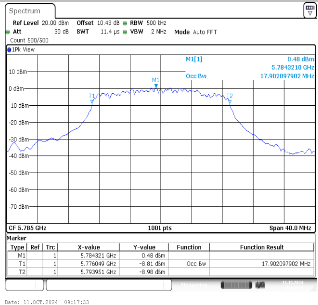
11AC20MIMO-Ant2-5785
