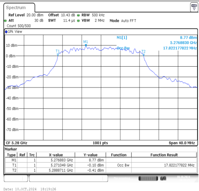
11AC20MIMO-Ant2-5280
