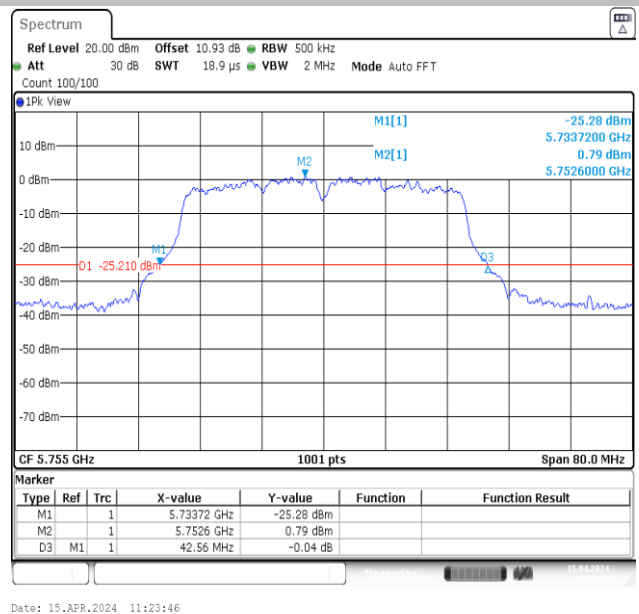
11N40MIMO-Ant2-5755
