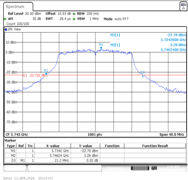
11A-Ant2-5745
