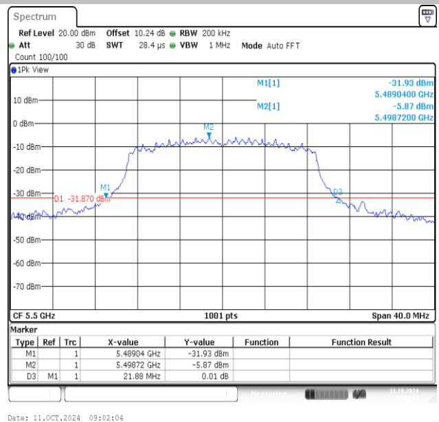
11AC20MIMO-Ant2-5500
