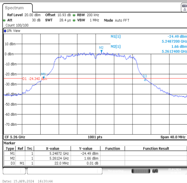
11N20MIMO-Ant2-5260
