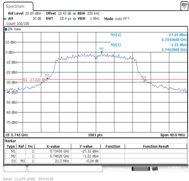
11AC20MIMO-Ant2-5745
