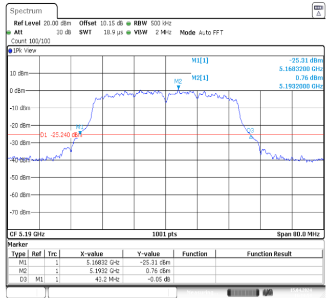
11N40MIMO-Ant2-5190
