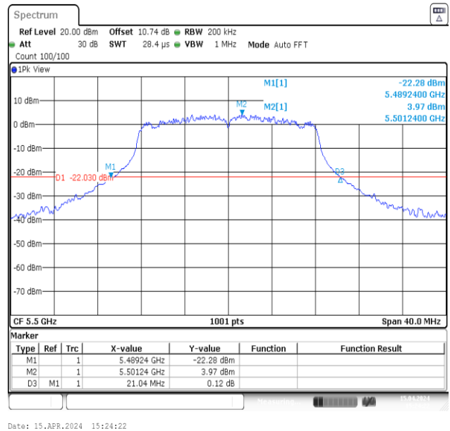
11A-Ant2-5500
