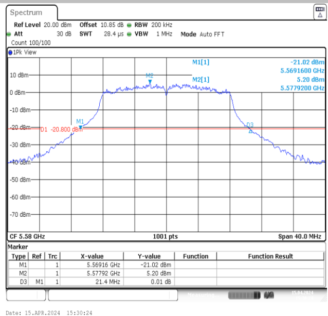
11A-Ant2-5580
