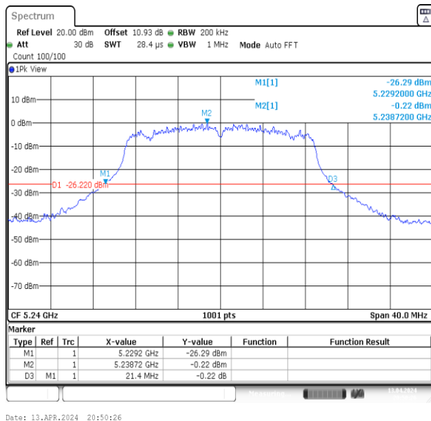
11N20MIMO-Ant2-5240
