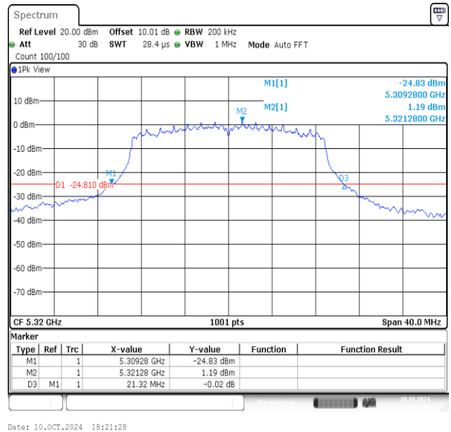
11AC20MIMO-Ant2-5320
