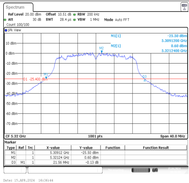
11N20MIMO-Ant2-5320
