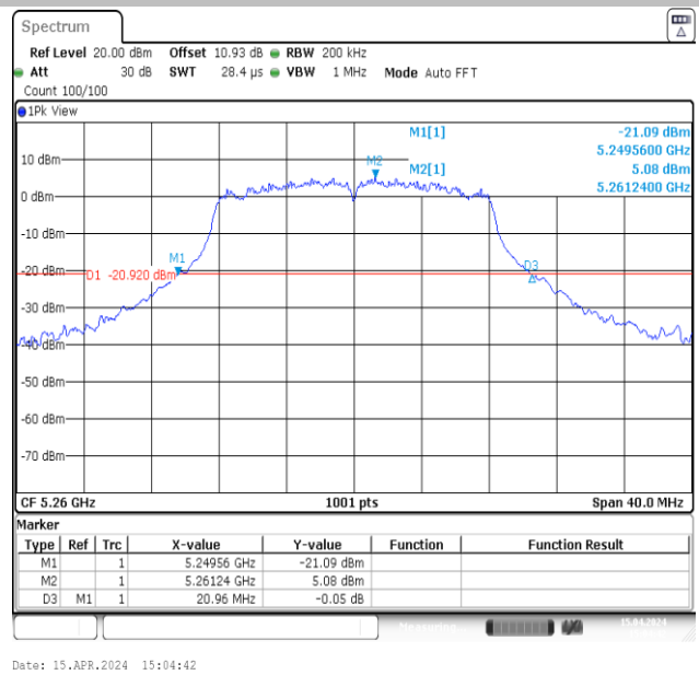
11A-Ant2-5260
