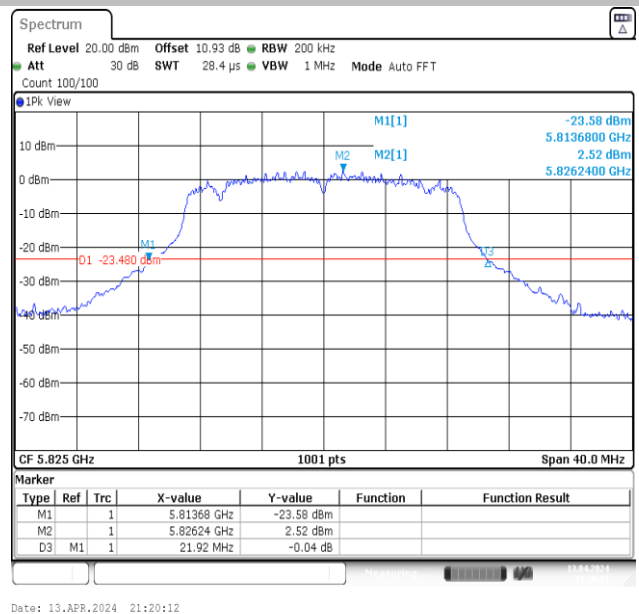
11N20MIMO-Ant2-5825
