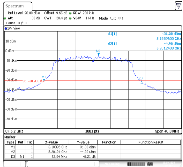
11AC20MIMO-Ant2-5200
