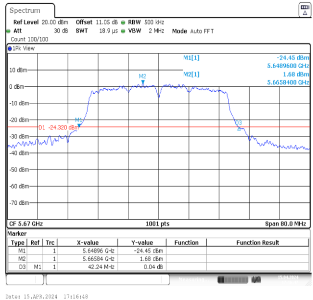
11N40MIMO-Ant2-5670
