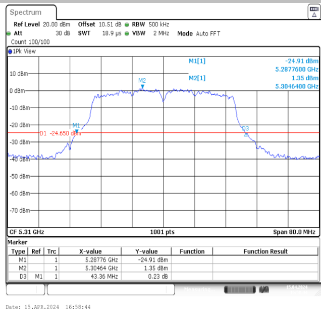
11N40MIMO-Ant2-5310
