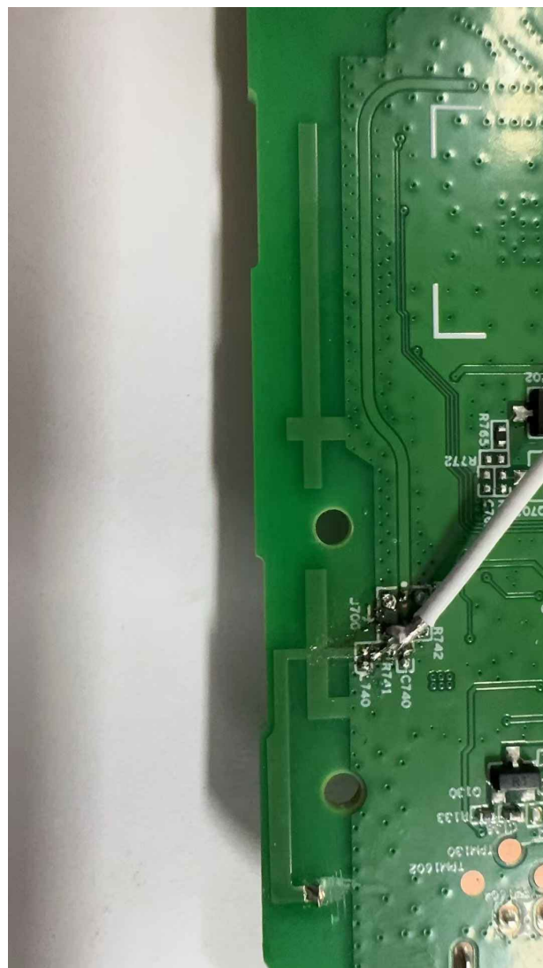
Picture 4 (WIFIB Antenna)
