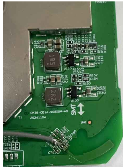
Picture6 (BT Antenna)
