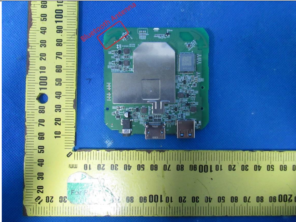
EUT Photo(10) Bluetooth Antenna
