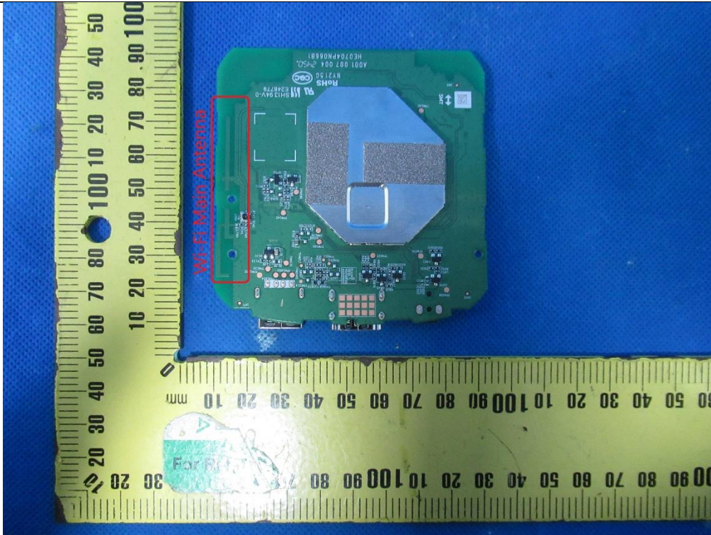
EUT Photo(8) Wi-Fi Antenna
