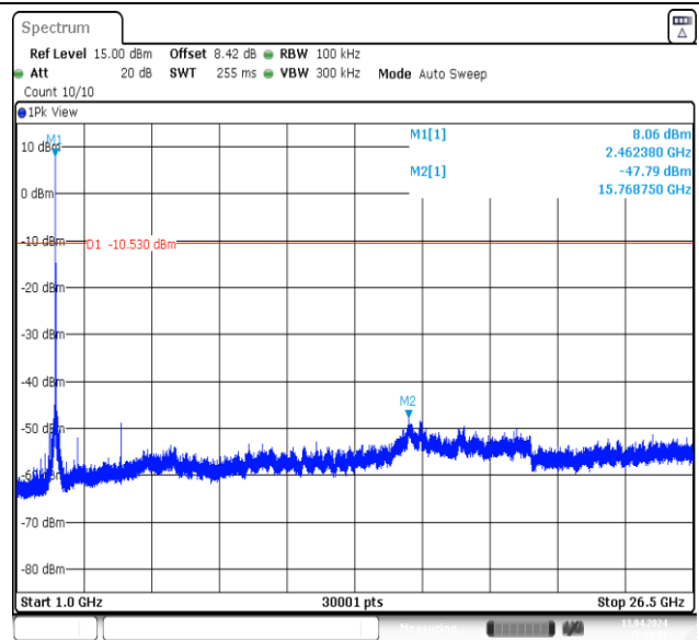
11B-Ant2-2462-1000~26500-PASS
