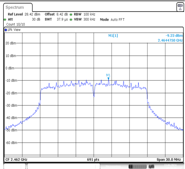
11N20MIMO-Ant2-2462-0~Reference-PASS
