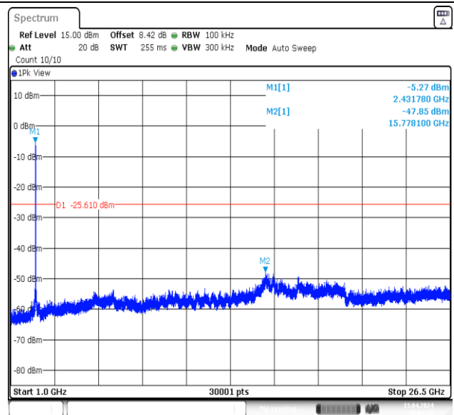
11N40MIMO-Ant2-2437-1000~26500-PASS
