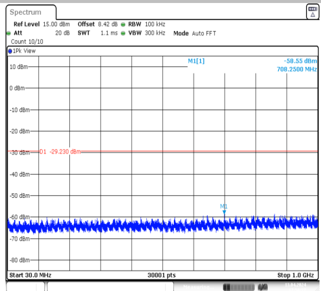
11N20MIMO-Ant2-2462-0~Reference-PASS
