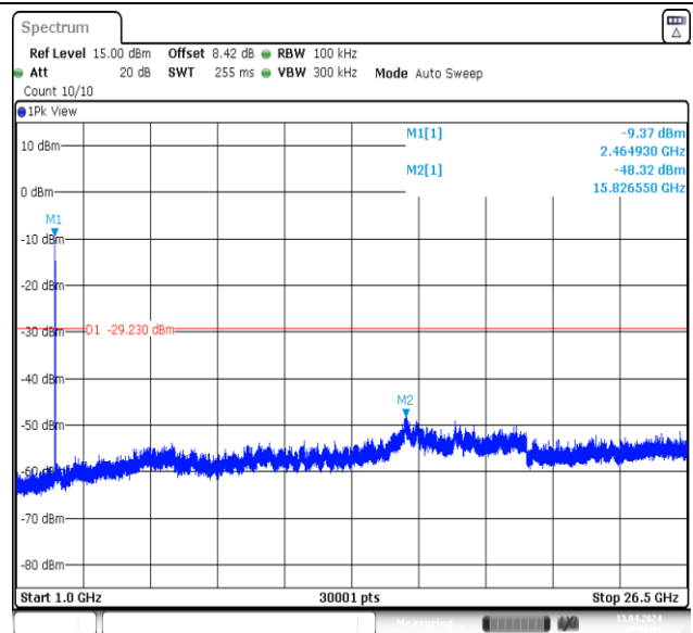
11N20MIMO-Ant2-2462-1000~26500-PASS
