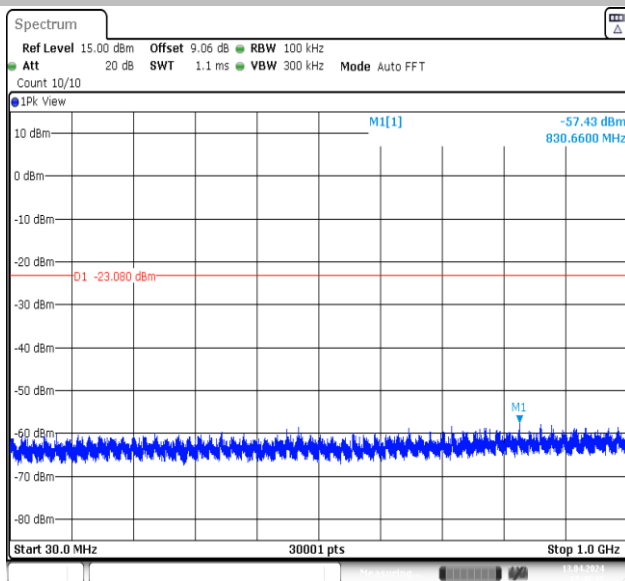
11N20MIMO-Ant1-2462-0~Reference-PASS
