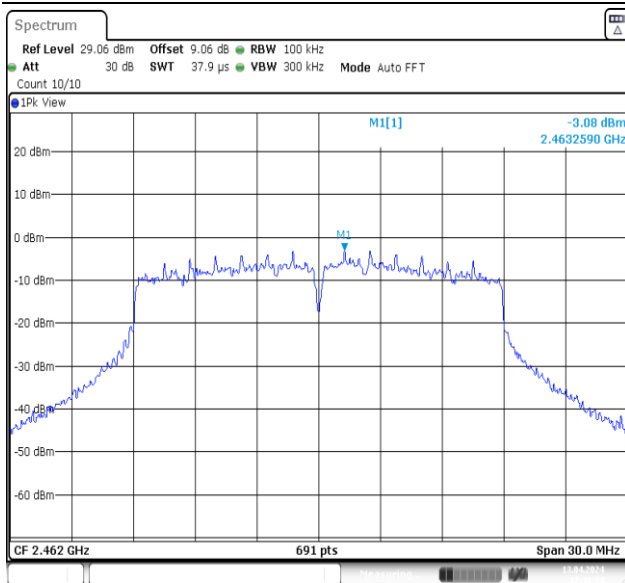
11N20MIMO-Ant1-2462-0~Reference-PASS
