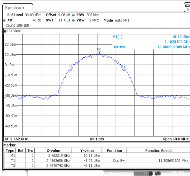
11B-Ant1-2462
