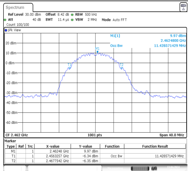
11B-Ant2-2462
