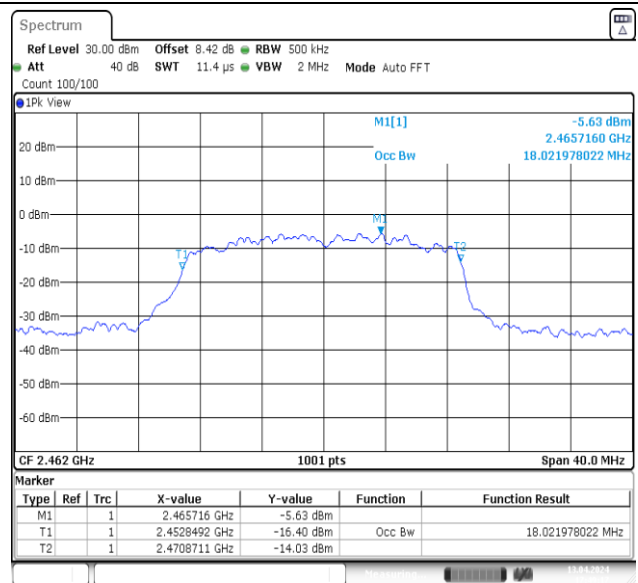
11N20MIMO-Ant2-2462
