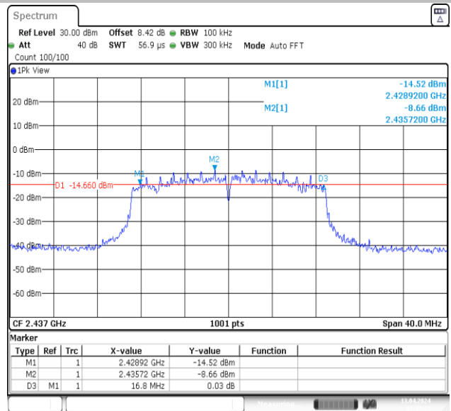
11N20MIMO-Ant2-2437-PASS
