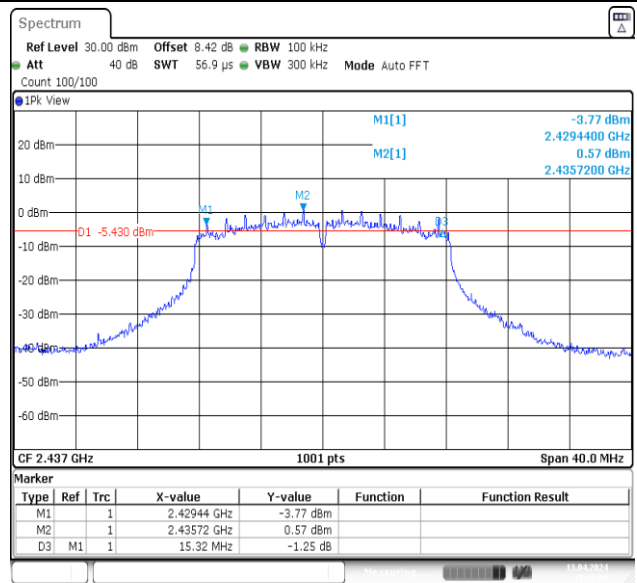
11G-Ant2-2437-PASS
