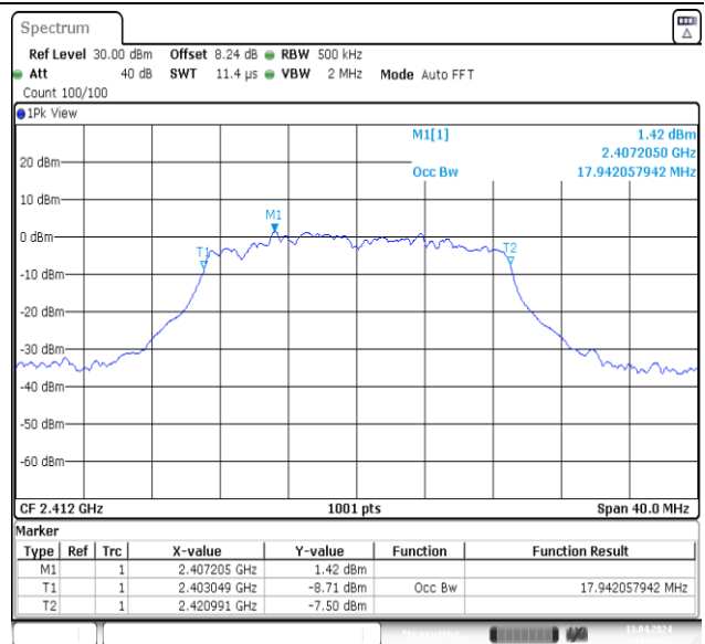
11N20MIMO-Ant2-2412
