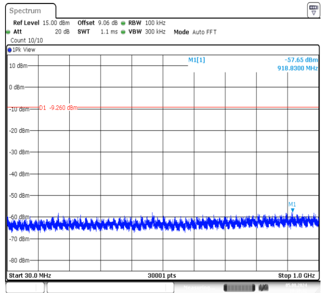
2DH5-Ant1-2441-30~1000-PASS
