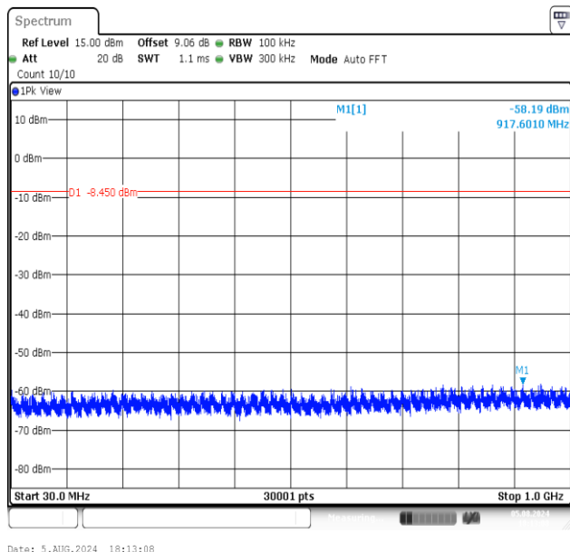
2DH5-Ant1-2480-30~1000-PASS
