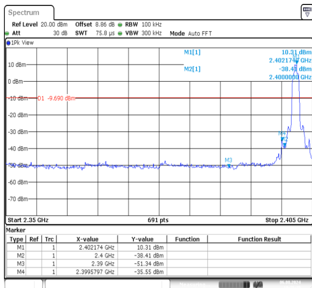
3DH5-Ant1-2402-PASS
