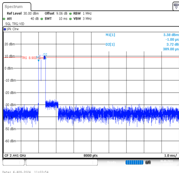
3DH1-Ant1-Hop-PASS
