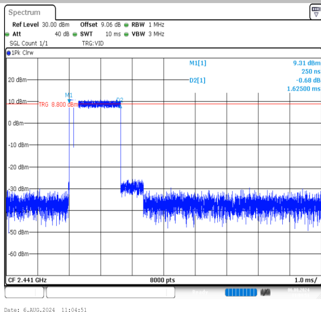
3DH3-Ant1-Hop-PASS
