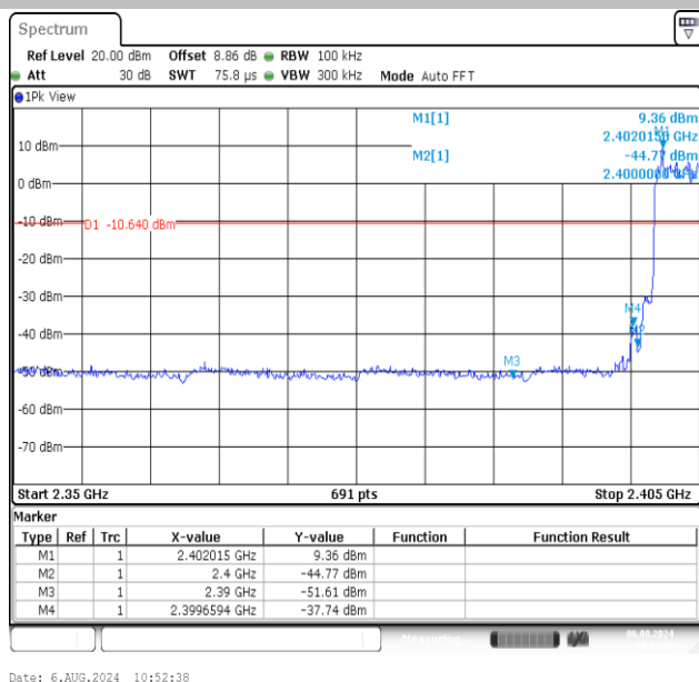
3DH5-Ant1-Hop_2402-PASS
