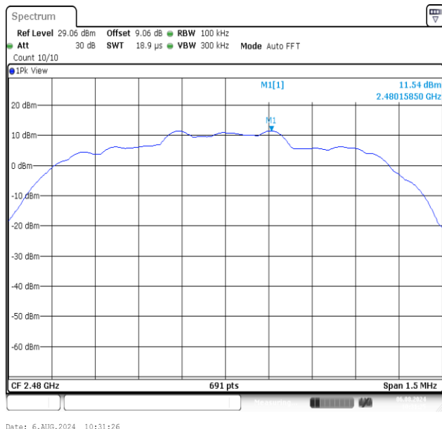
3DH5-Ant1-2480-0~Reference-PASS
