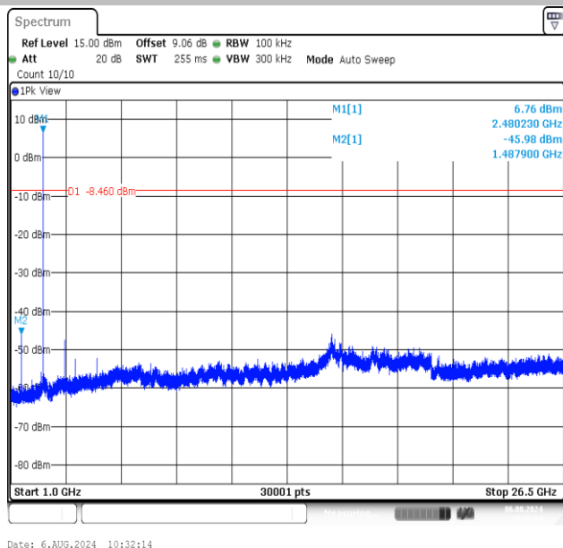
3DH5-Ant1-2480-1000~26500-PASS
