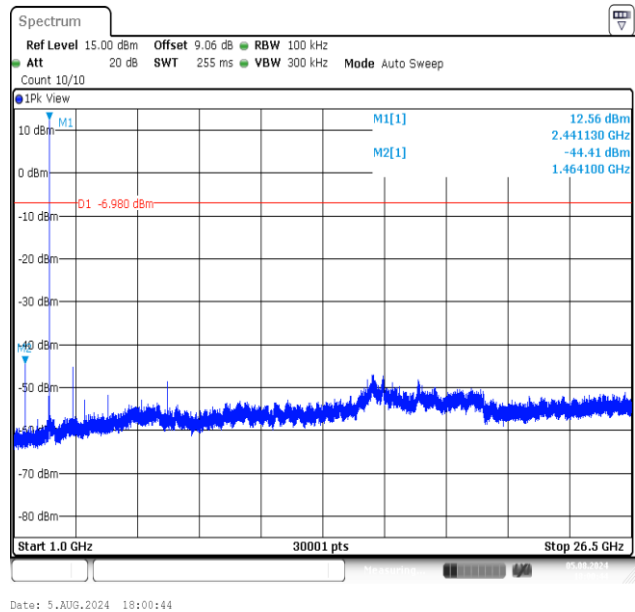
DH5-Ant1-2441-1000~26500-PASS
