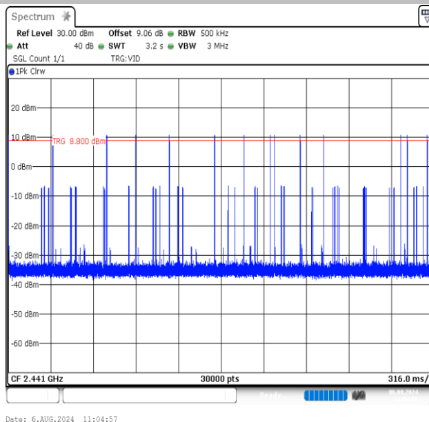
3DH3-Ant1-Hop-PASS
