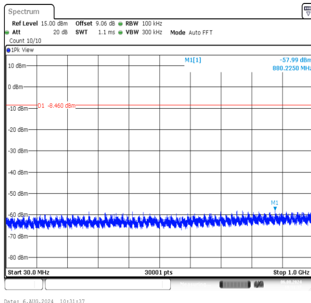
3DH5-Ant1-2480-30~1000-PASS
