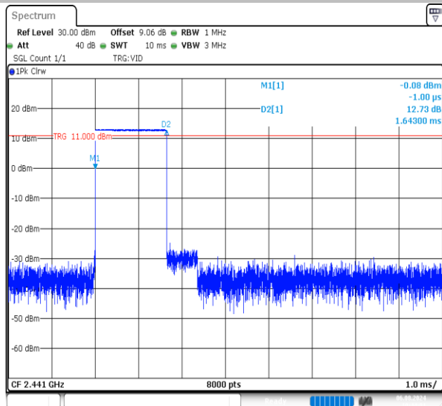
DH1-Ant1-Hop-PASS
