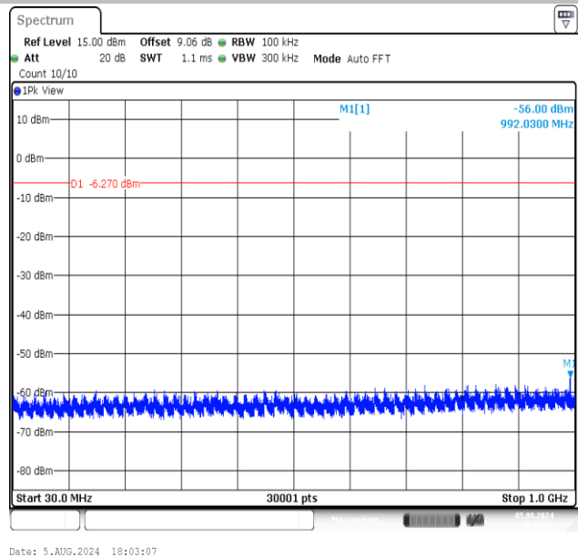
DH5-Ant1-2480-30~1000-PASS
