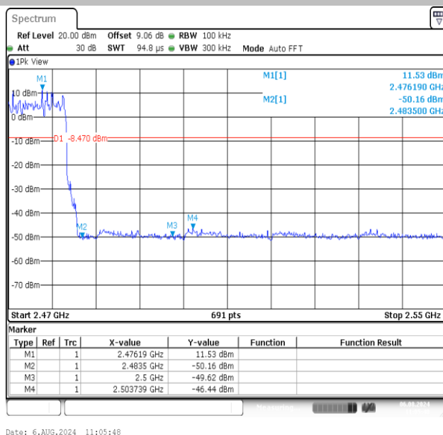
3DH5-Ant1-Hop_2480-PASS
