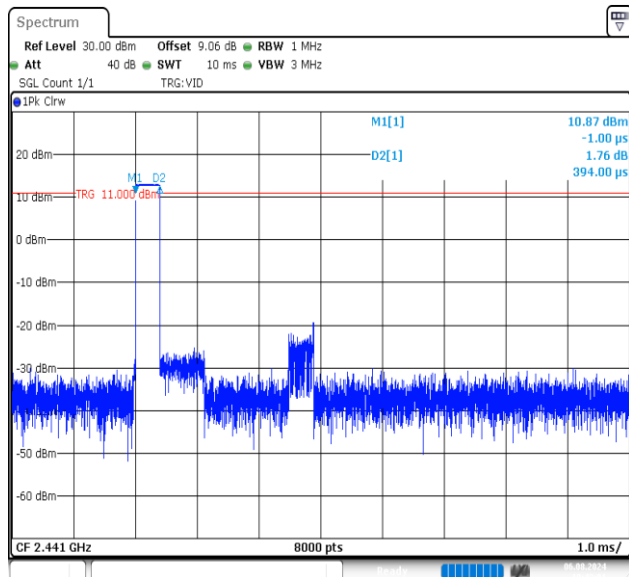
DH1-Ant1-Hop-PASS
