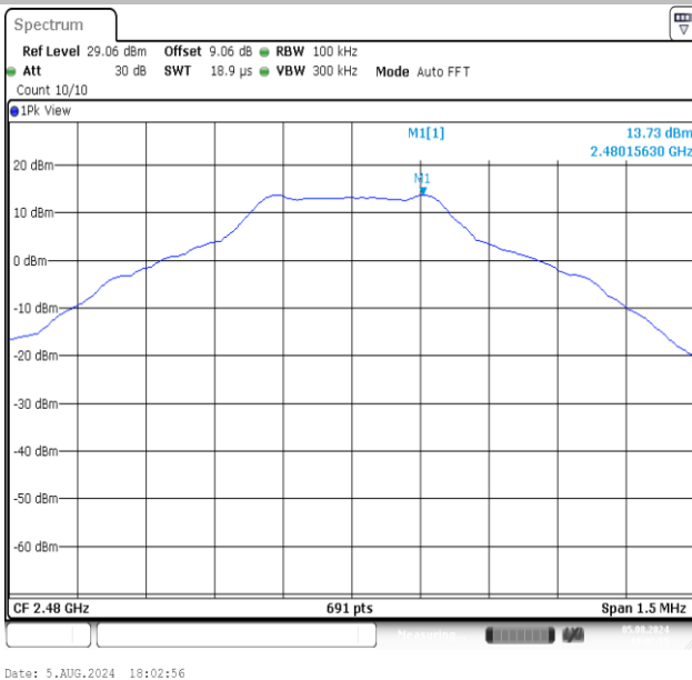
DH5-Ant1-2480-0~Reference-PASS
