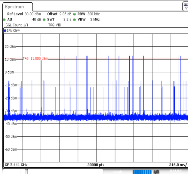
DH1-Ant1-Hop-PASS
