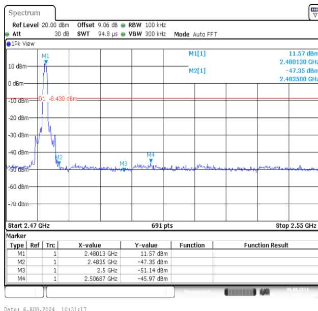
3DH5-Ant1-2480-PASS
