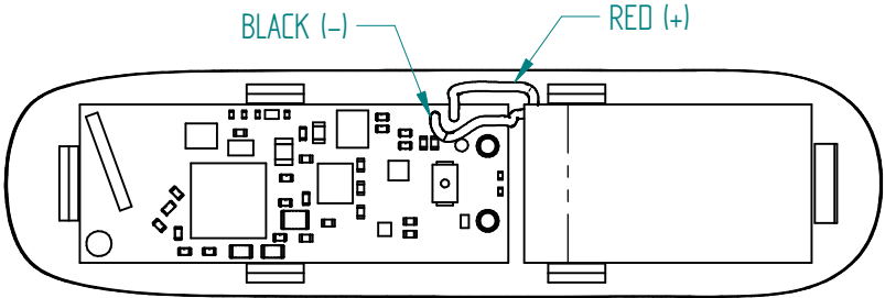
TOP VIEW OF WIRE ROUTING
