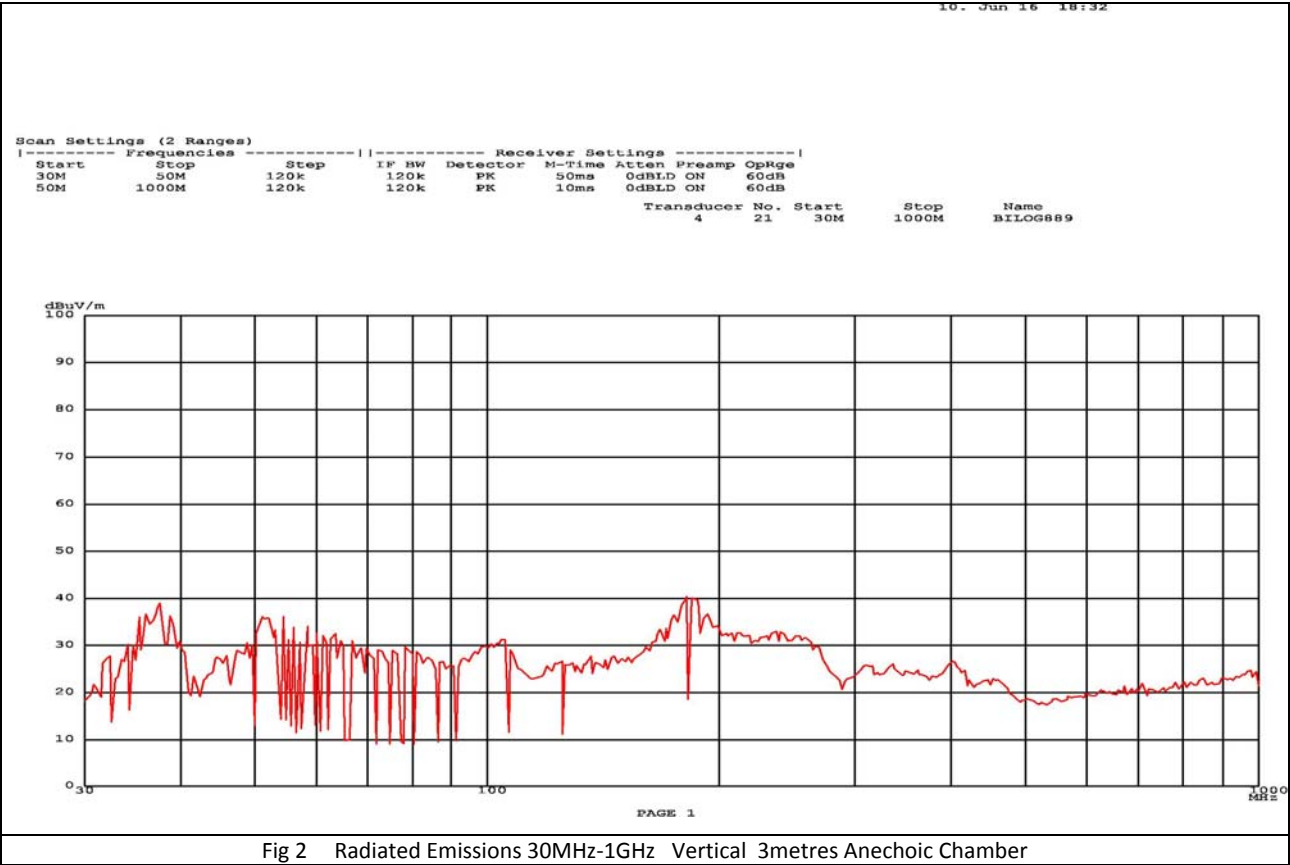
Fig 2 Radiated Emissions 30MHz-1GHz Vertical 3metres Anechoic Chamber
