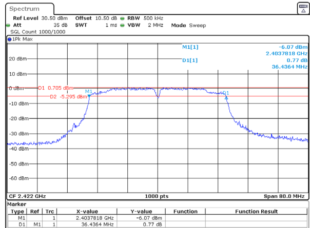
802.11n40_2422MHz_Chain 1
