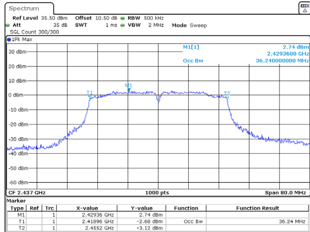
802.11n40_2437MHz_Chain 0
