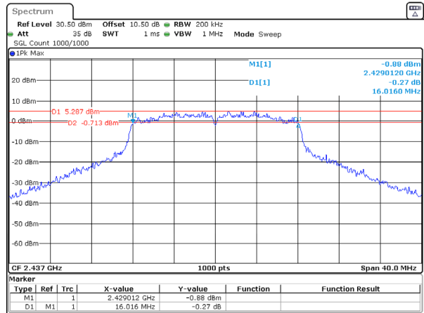
802.11g_2437MHz_Chain 0
