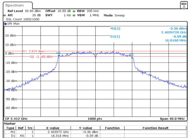
802.11g_2412MHz_Chain 1
