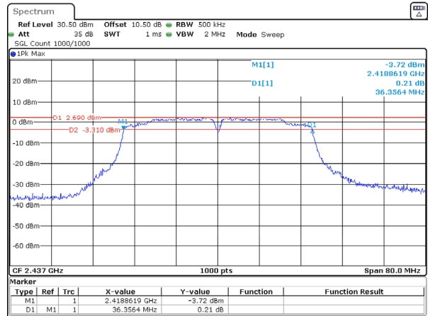
802.11n40_2437MHz_Chain 0
