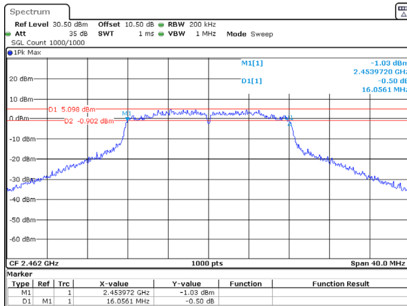
802.11g_2462MHz_Chain 0
