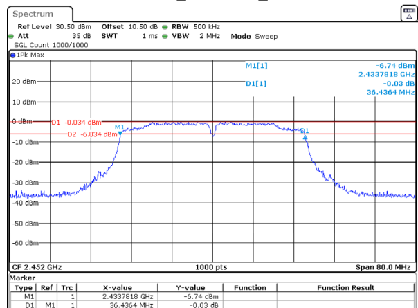
802.11n40_2452MHz_Chain 1
