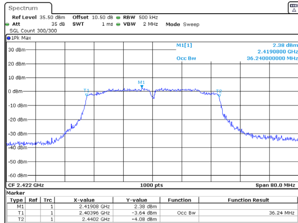
802.11n40_2422MHz_Chain 0
