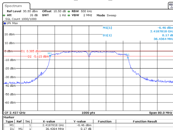
802.11n40_2437MHz_Chain 1
