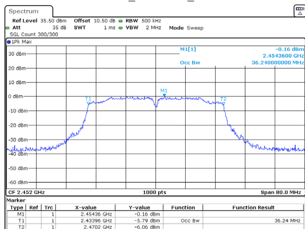
802.11n40_2452MHz_Chain 1
