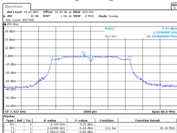
802.11n40_2437MHz_Chain 1
