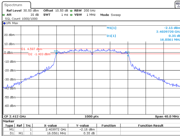
802.11g_2412MHz_Chain 0
