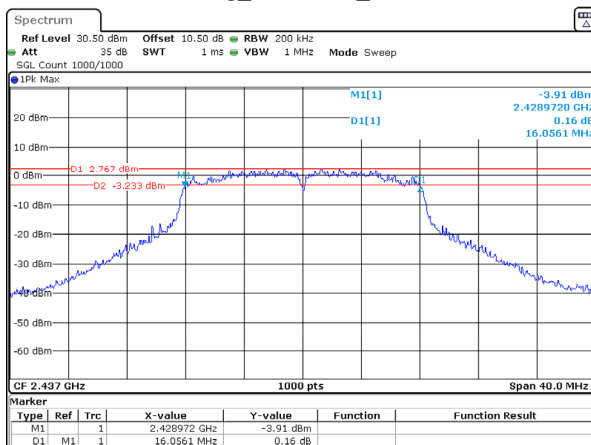
802.11g_2437MHz_Chain 1
