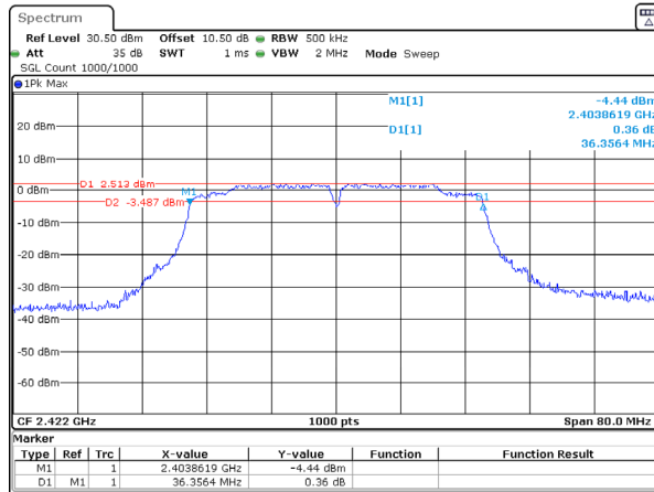
802.11n40_2422MHz_Chain 0
