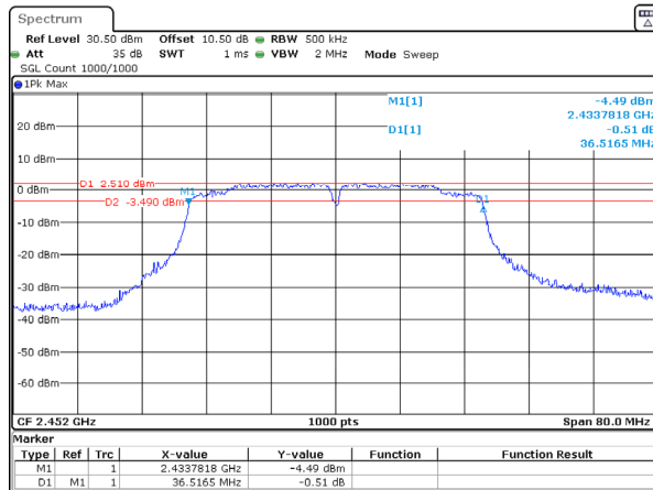
802.11n40_2452MHz_Chain 0
