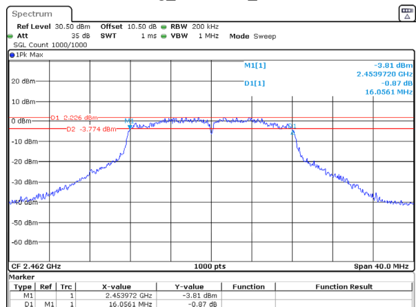
802.11g_2462MHz_Chain 1
