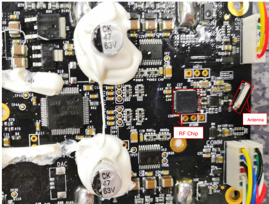
MAIN BOARD TOP VIEW (CLOSE-UP 1)
