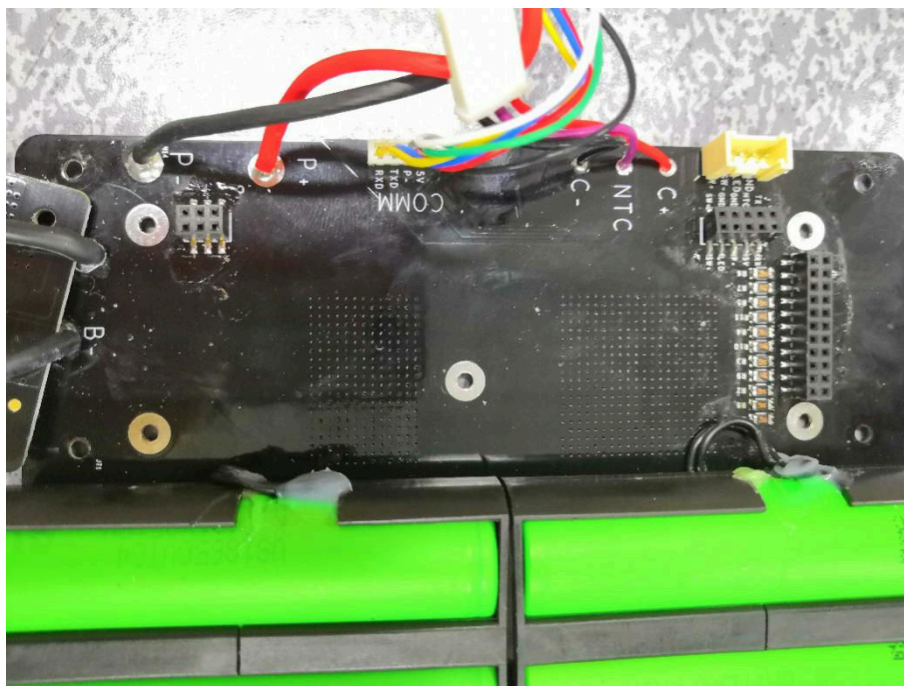
MAIN BOARD TOP VIEW (CLOSE-UP 3)
