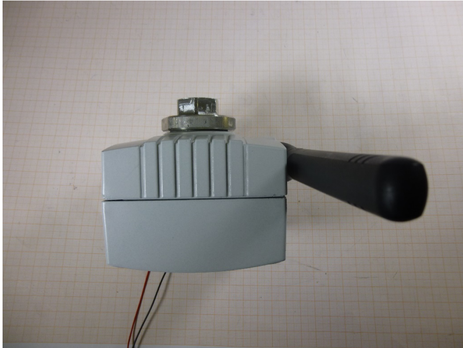
Photo 11: EUT top side view, metal housing (ex version)
