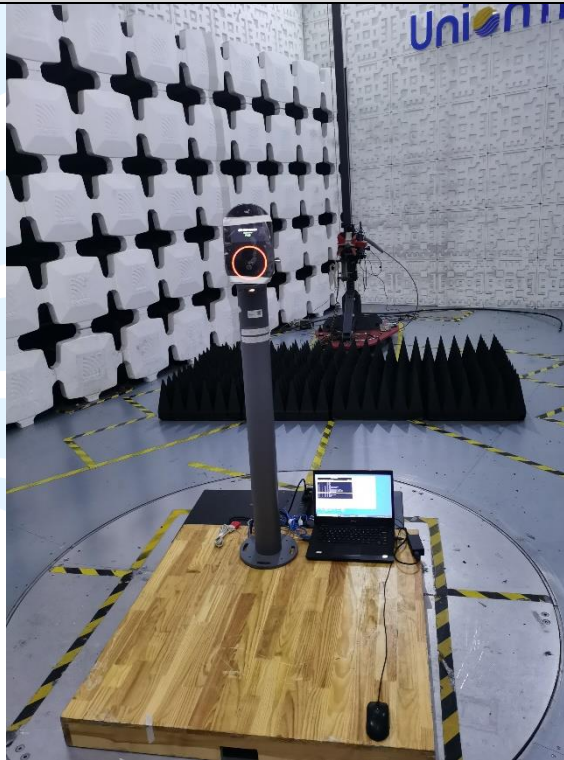
Radiated emission Test Setup-2 (Above 1 GHz)
