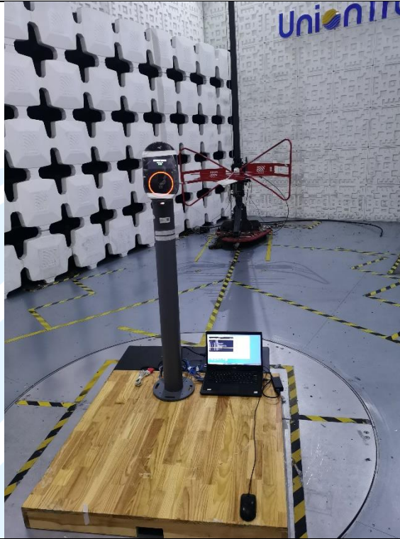
Radiated emission Test Setup-1 (30 MHz~1 GHz)
