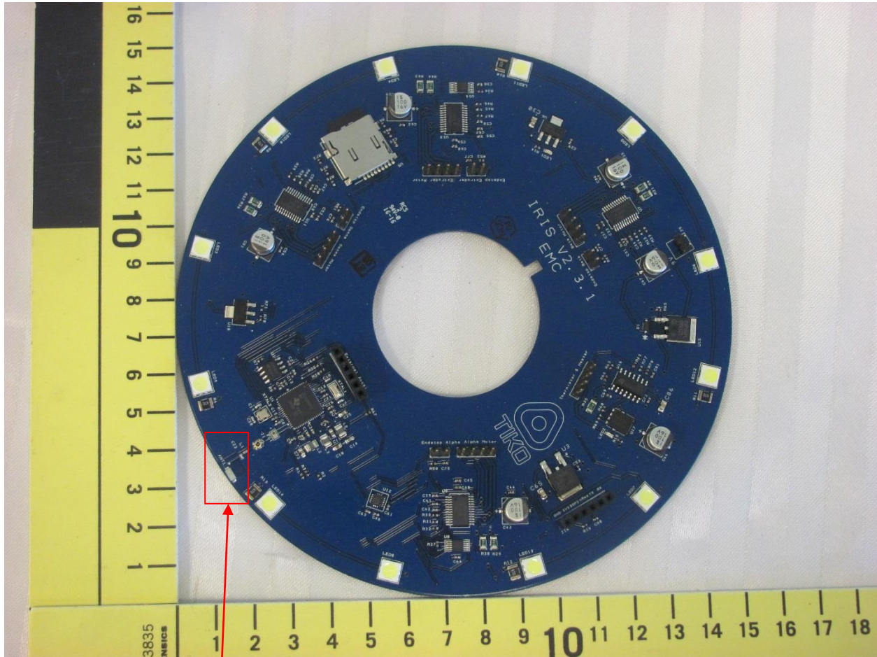
Figure 4: Internal view – PCB Top
