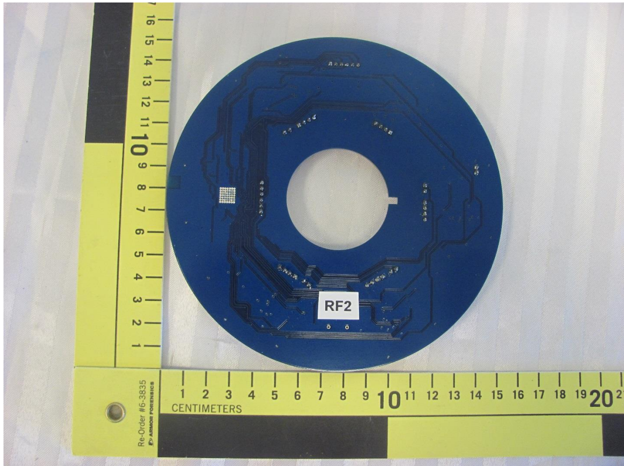
Figure 5: Internal view – PCB bottom
