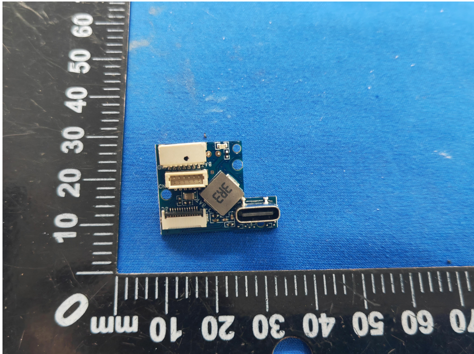
SECONDARY BOARD 1 REAR VIEW
