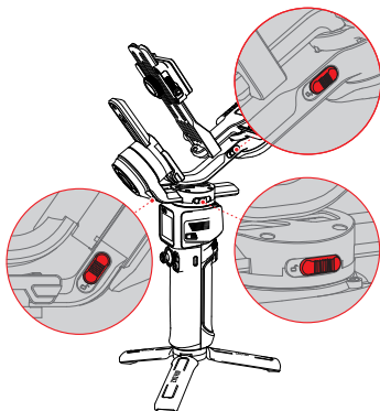
Lock state for storage
