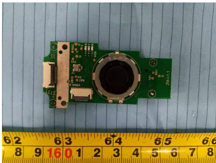
EUT – Small Board 5 Top View
