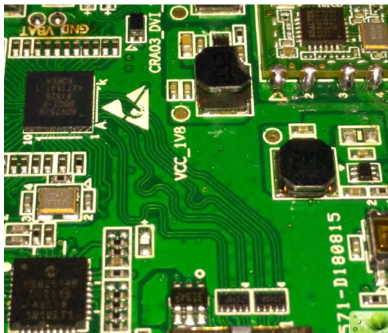
EUT – Main Board 1 IC Chip View
