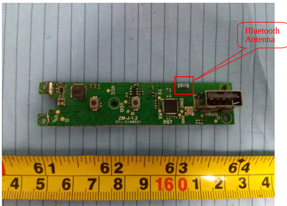
EUT – Main Board 4 Top Cover off View
