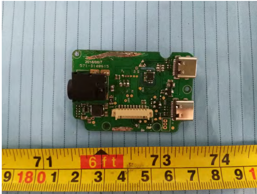
EUT – Main Board 3 Top Cover off View
