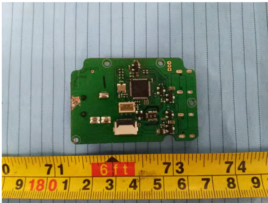
EUT – Main Board 3 Bottom Cover off View
