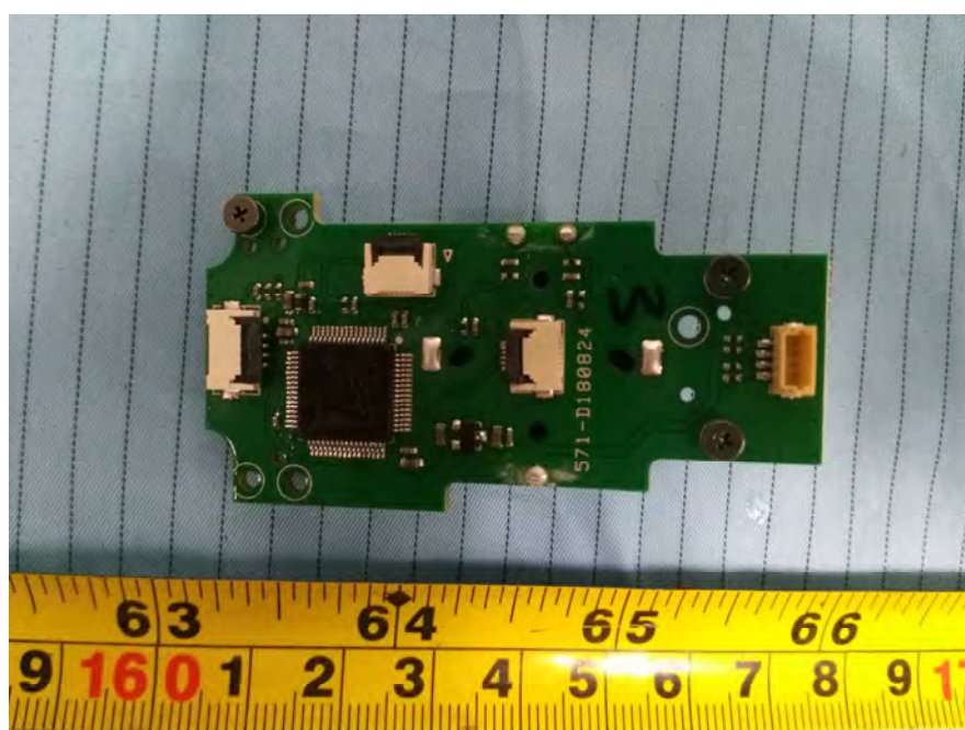
EUT – Small Board 5 Bottom View
