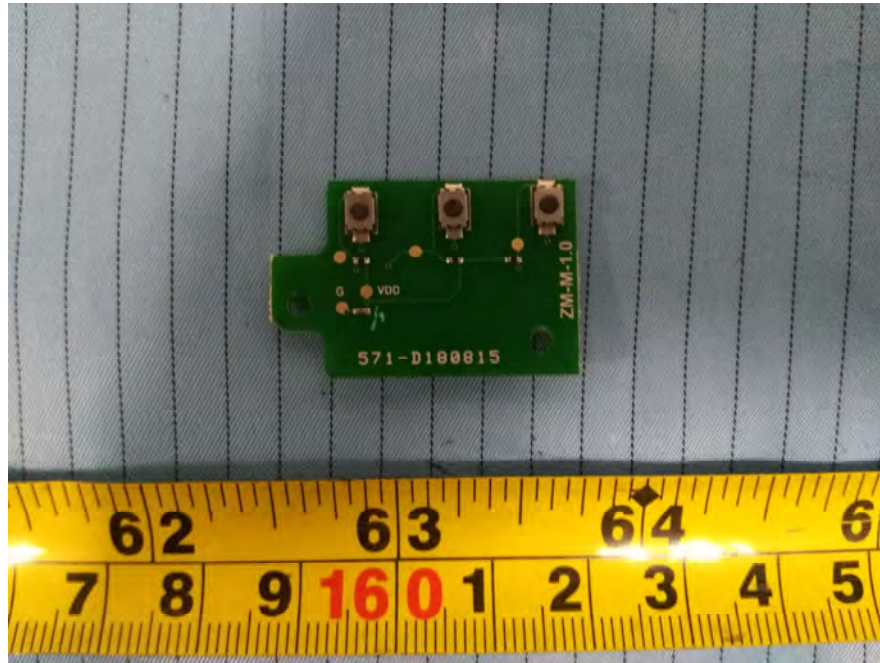
EUT – Small Board 10 Top View
