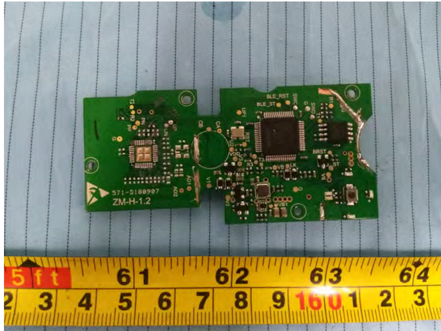
EUT – Main Board 5 Top Cover off View
