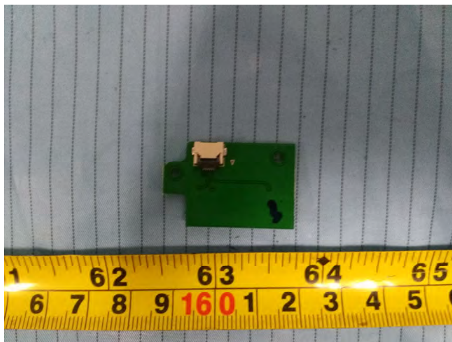
EUT – Small Board 10 Bottom View
