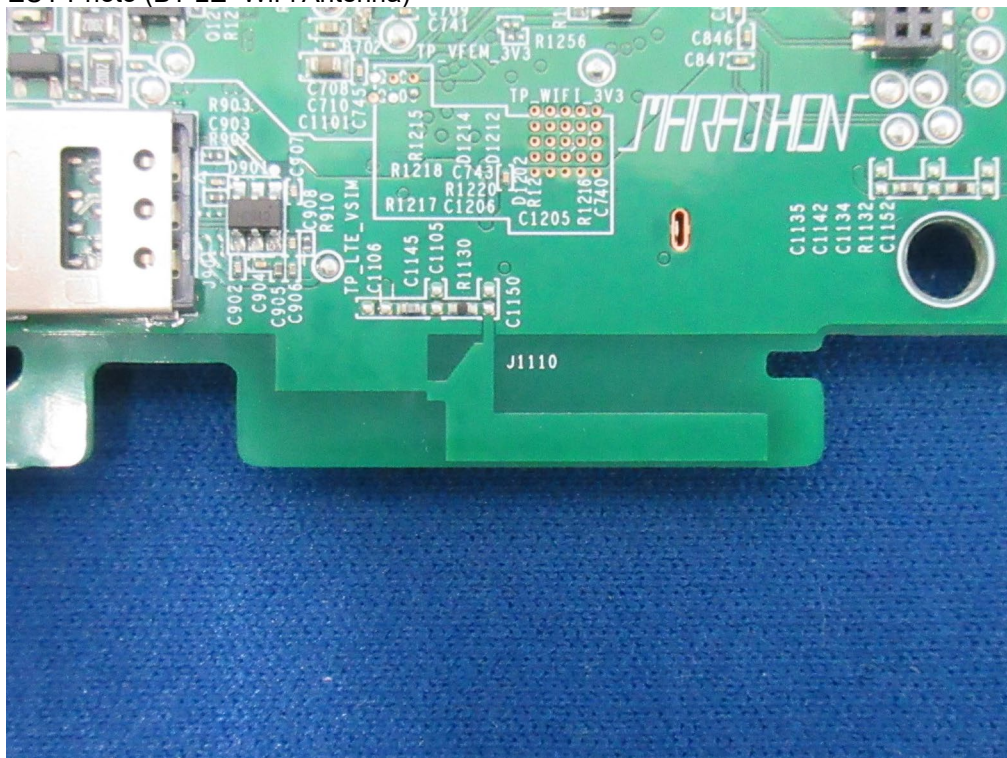
(8) EUT Photo (BT LE+WiFi Antenna)
