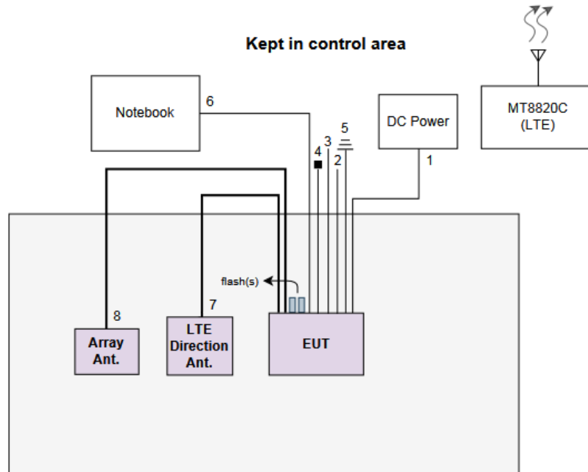
Test Setup Diagram (Directional antenna)
