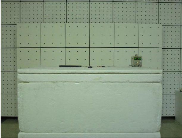
Part_15_247_LE_Radiated_966 (2)_Setup
