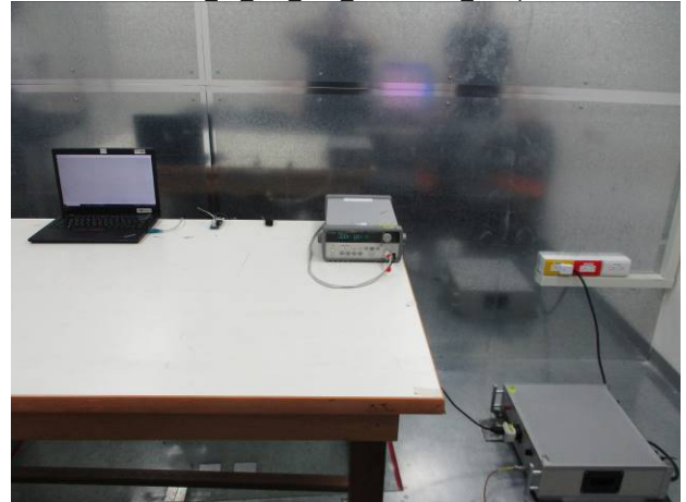
FCC 15 247 BLE Conduction Setup
