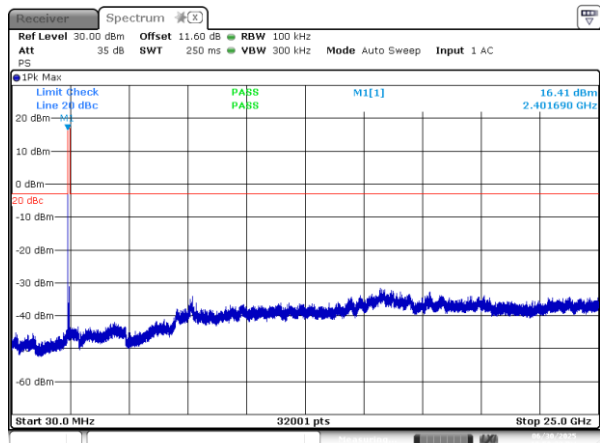
Figure 7.6-7: Conducted spurious emissions on low channel
