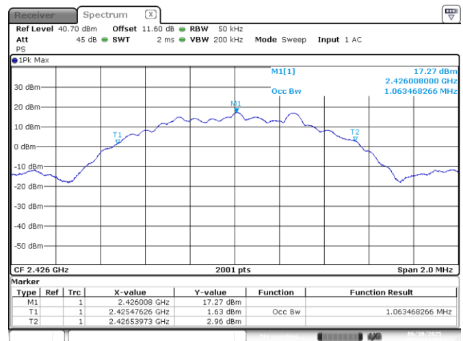
Figure 7.4-2: 99% bandwidth – sample plot
