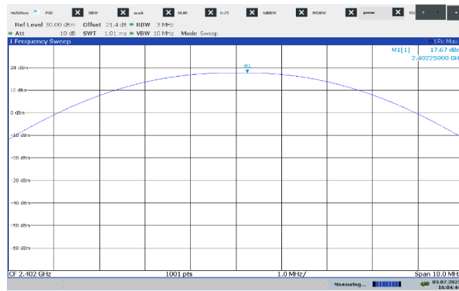
Figure 7.5-1: Output power on low channel
