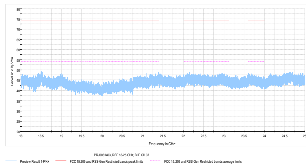
Figure 7.6-14: Radiated spurious emissions on Low channel, 18 – 25 GHz
