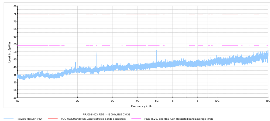
Figure 7.6-17: Radiated spurious emissions on high channel, 1 – 18 GHz
