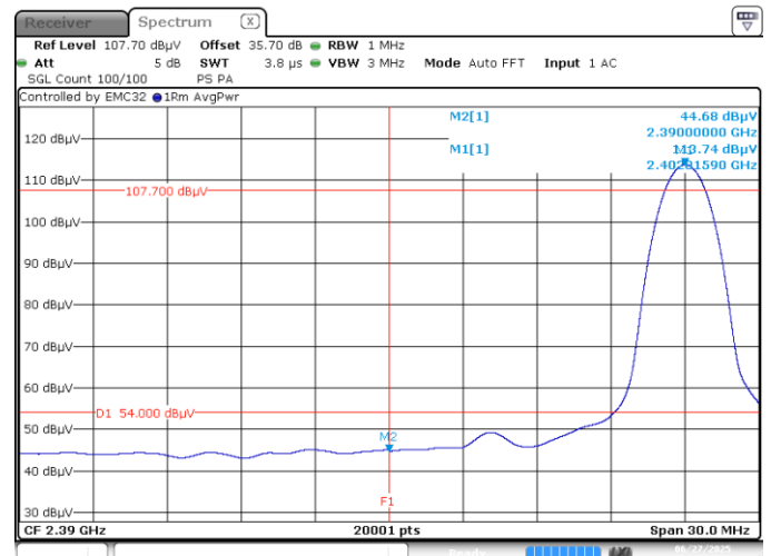
Figure 7.6-2: Restricted band edge spurious emissions at 2390 MHz, Average
