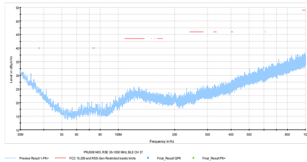
Figure 7.6-10: Radiated spurious emissions on Low channel, 30 – 1000 MHz
