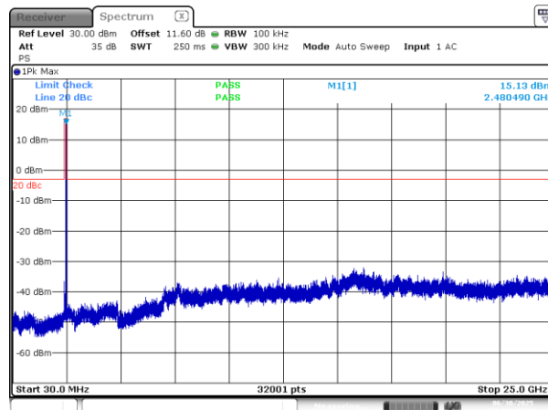
Figure 7.6-9: Conducted spurious emissions on high channel
