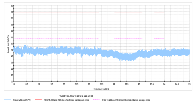
Figure 7.6-15: Radiated spurious emissions on Mid channel, 18 – 25 GHz
