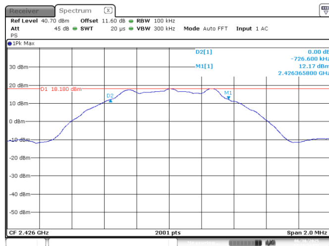
Figure 7.4-1: 6 dB bandwidth – sample plot
