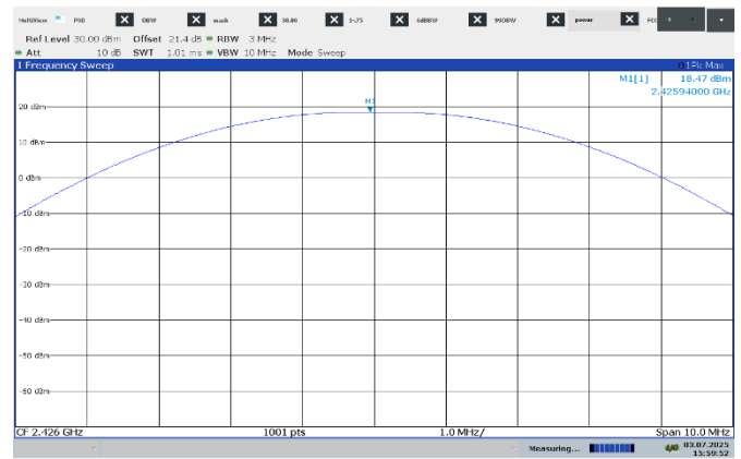
Figure 7.5-2: Output power on mid channel
