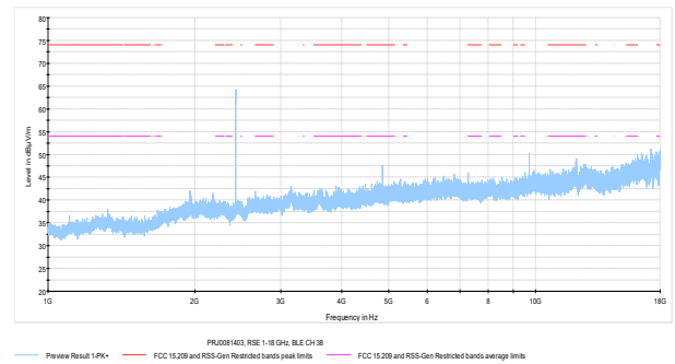
Figure 7.6-13: Radiated spurious emissions on Mid channel, 1 – 18 GHz
