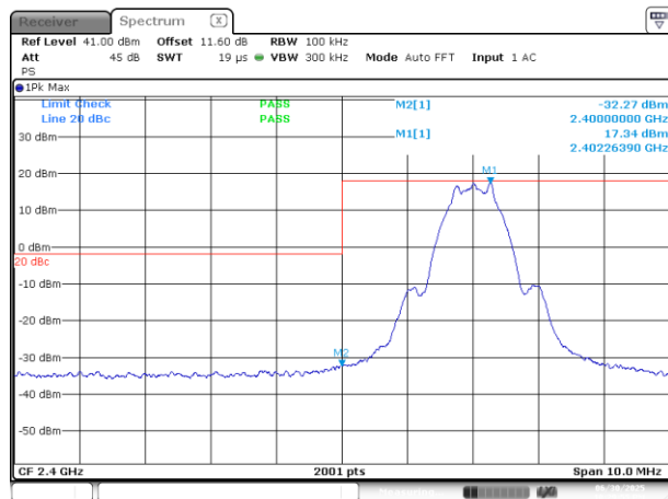
Figure 7.6-5: Conducted band edge spurious emissions at 2400 MHz
