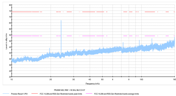
Figure 7.6-12: Radiated spurious emissions on Low channel, 1 – 18 GHz
