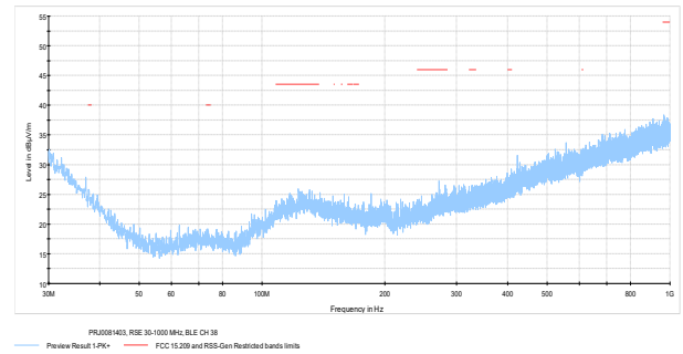
Figure 7.6-11: Radiated spurious emissions on Mid channel, 30 – 1000 MHz
