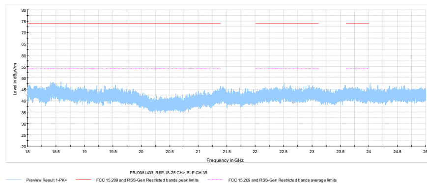
Figure 7.6-18: Radiated spurious emissions on high channel, 18 – 25 GHz
