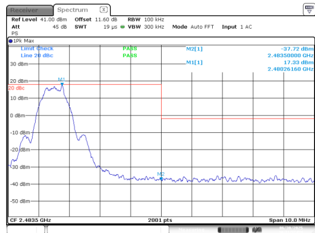
Figure 7.6-6: Conducted band edge spurious emissions at 2483.5 MHz
