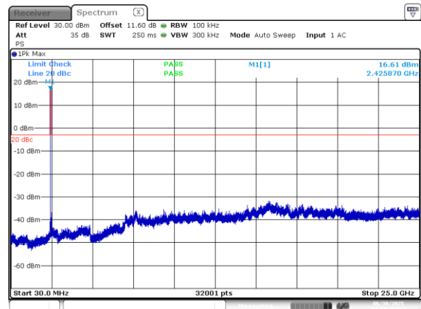
Figure 7.6-8: Conducted spurious emissions on mid channel
